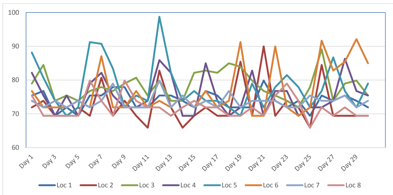
Figure 2. Summary of Construction Vibration Monitoring Data (VdB) – September 2016
