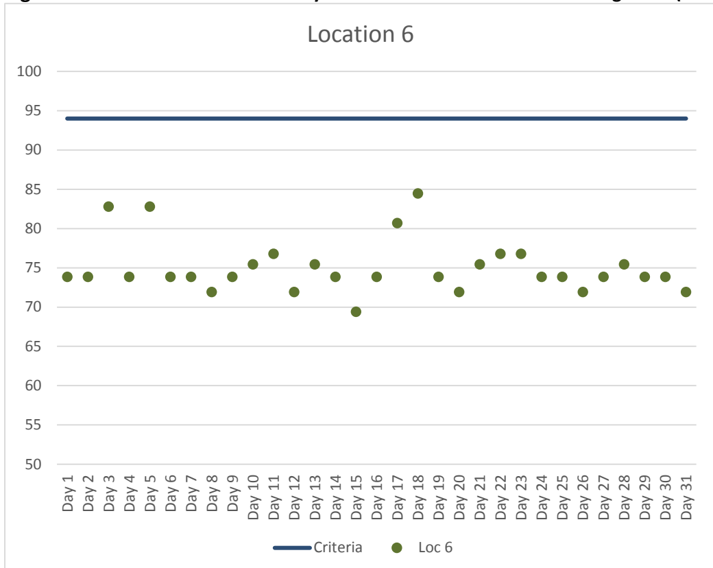
Figure 7. Location 6 Maximum Daily Construction Vibration Monitoring Data (VdB) – October 2017
