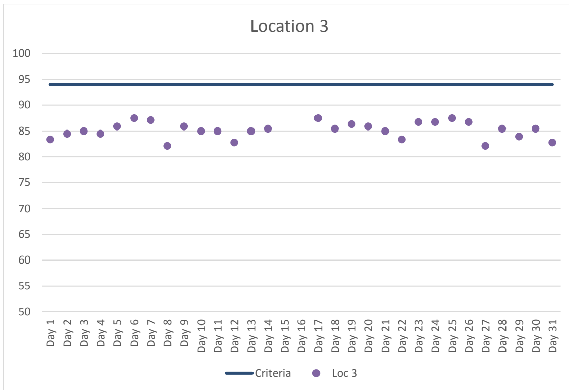
Figure 4. Location 3 Maximum Daily Construction Vibration Monitoring Data (VdB) – October 2017
