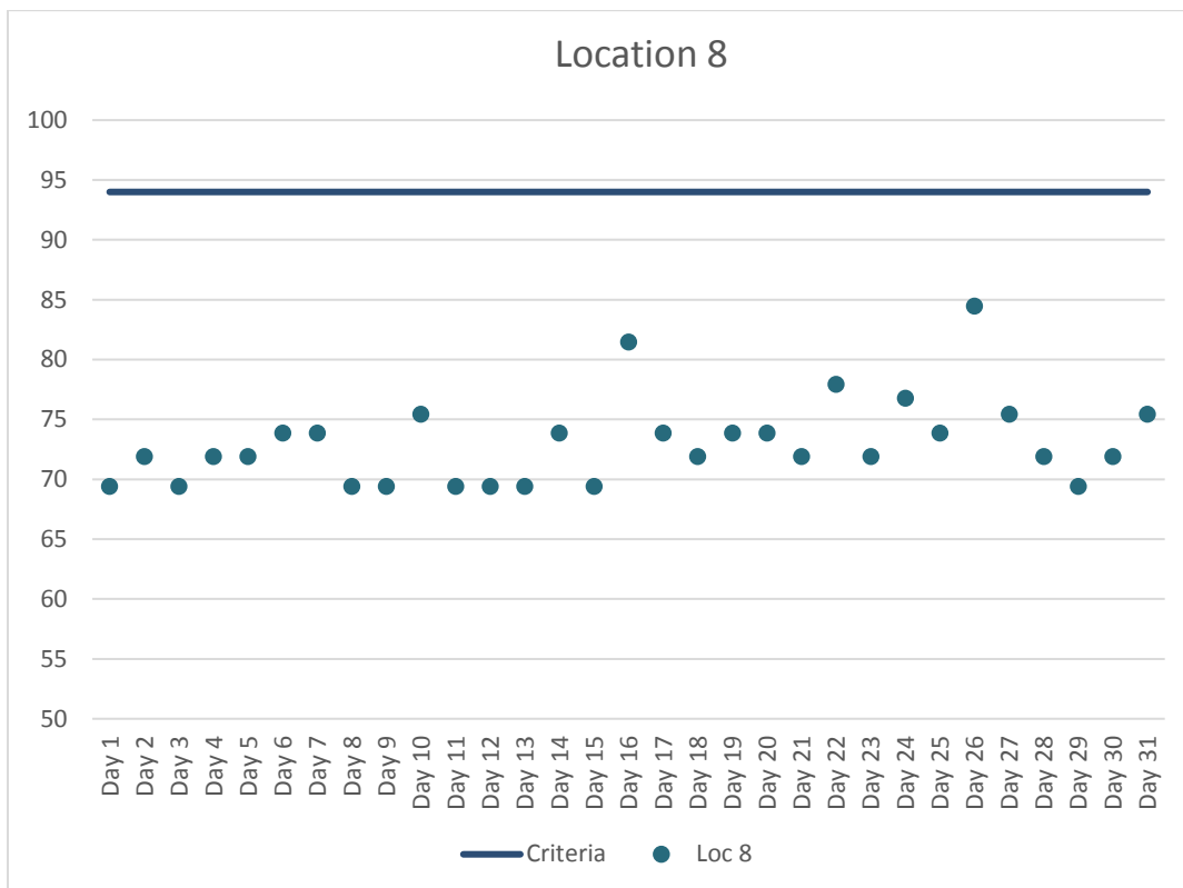
Figure 9. Location 8 Maximum Daily Construction Vibration Monitoring Data (VdB) – October 2017
