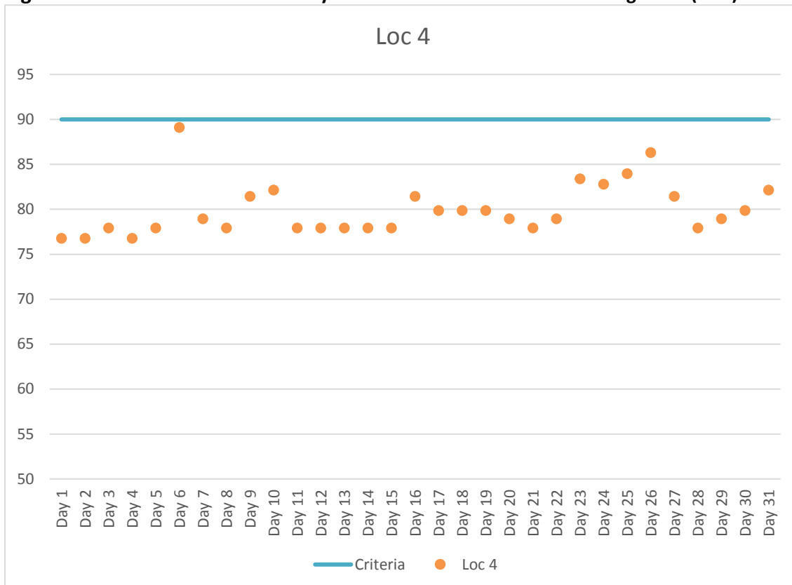
Figure 5. Location 4 Maximum Daily Construction Vibration Monitoring Data (VdB) – October 2017
