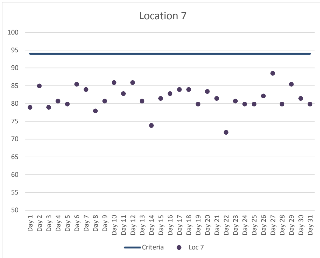
Figure 8. Location 7 Maximum Daily Construction Vibration Monitoring Data (VdB) – October 2017
