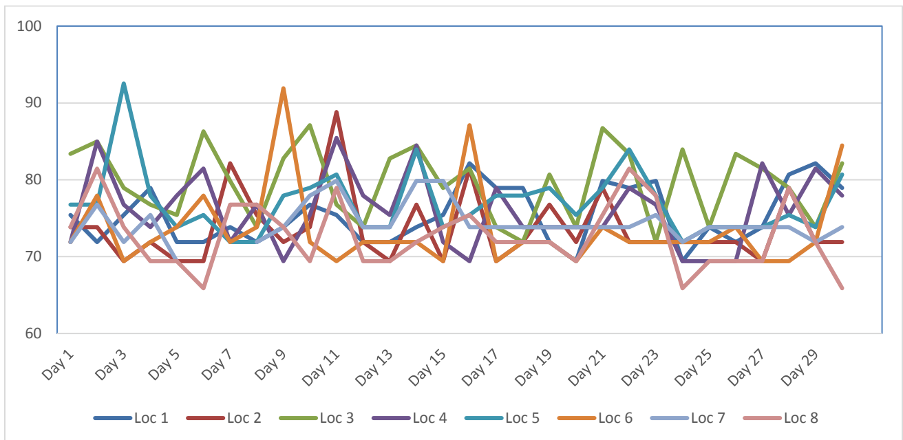
Figure 2. Summary of Construction Vibration Monitoring Data (VdB) – November 2016
