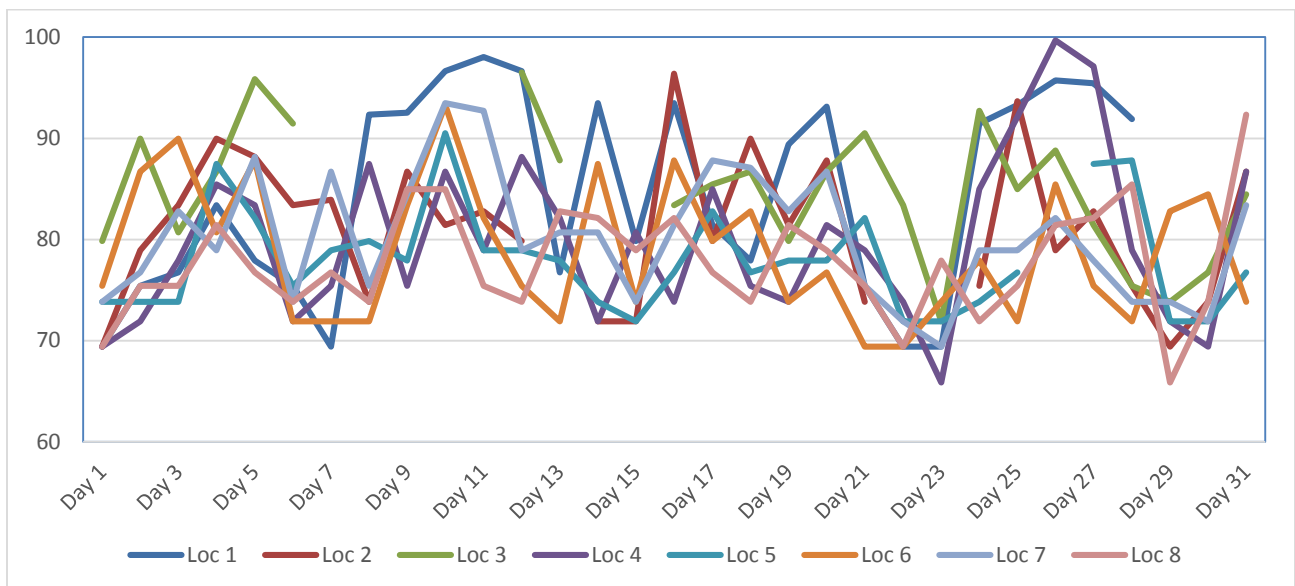
Figure 2. Summary of Construction Vibration Monitoring Data (VdB) – May 2016
