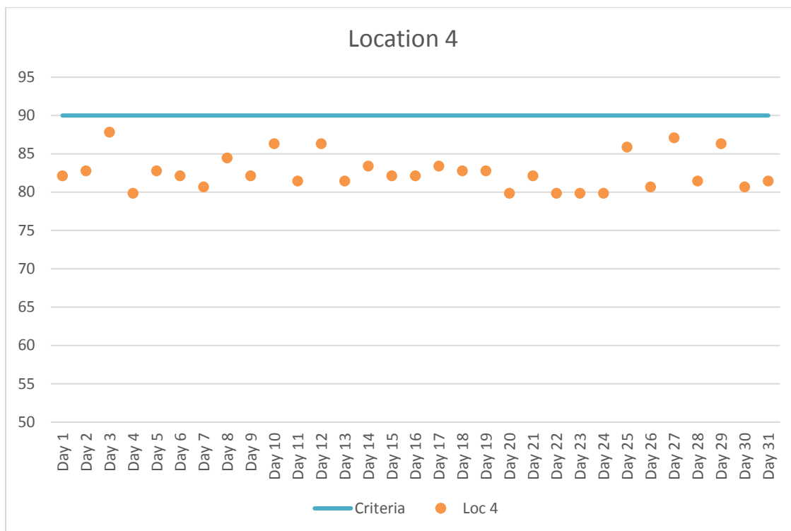
Figure 5. Location 4 Maximum Daily Construction Vibration Monitoring Data (VdB) –March 2018
