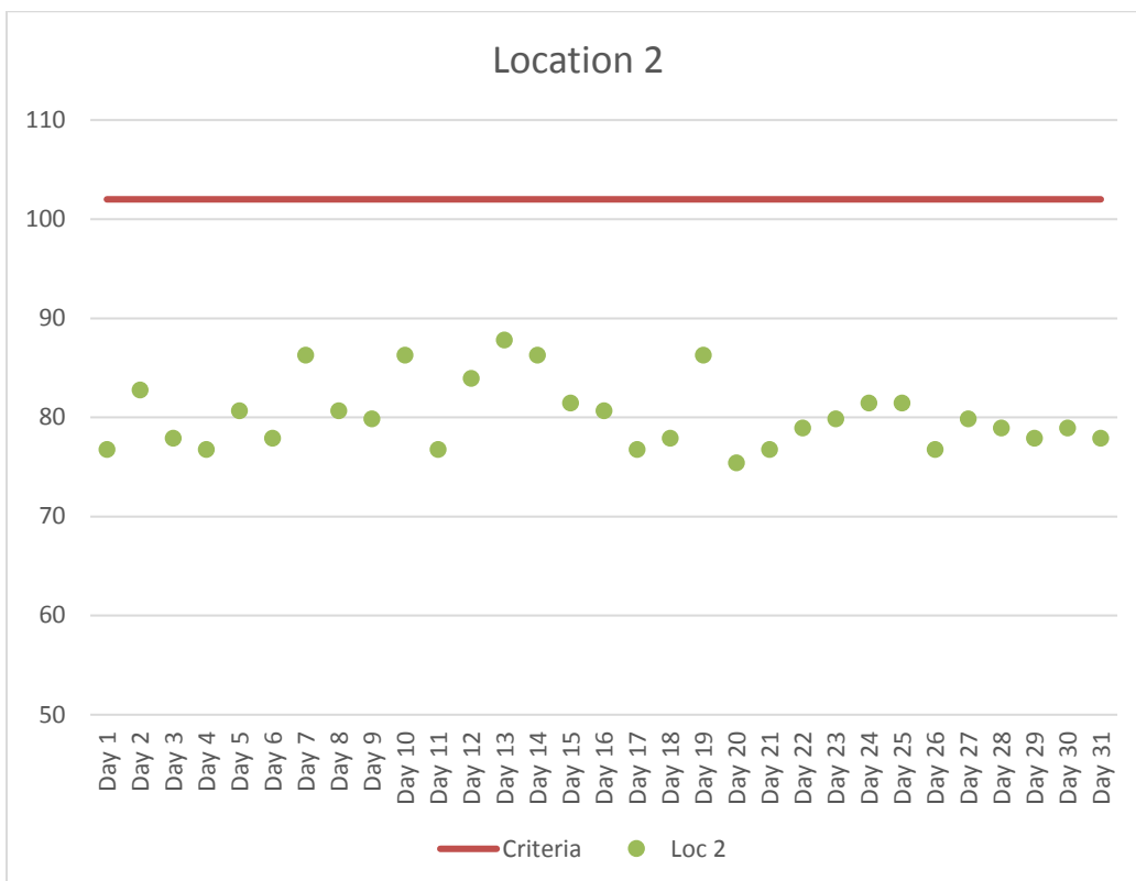
Figure 3. Location 2 Maximum Daily Construction Vibration Monitoring Data (VdB) – March 2018
