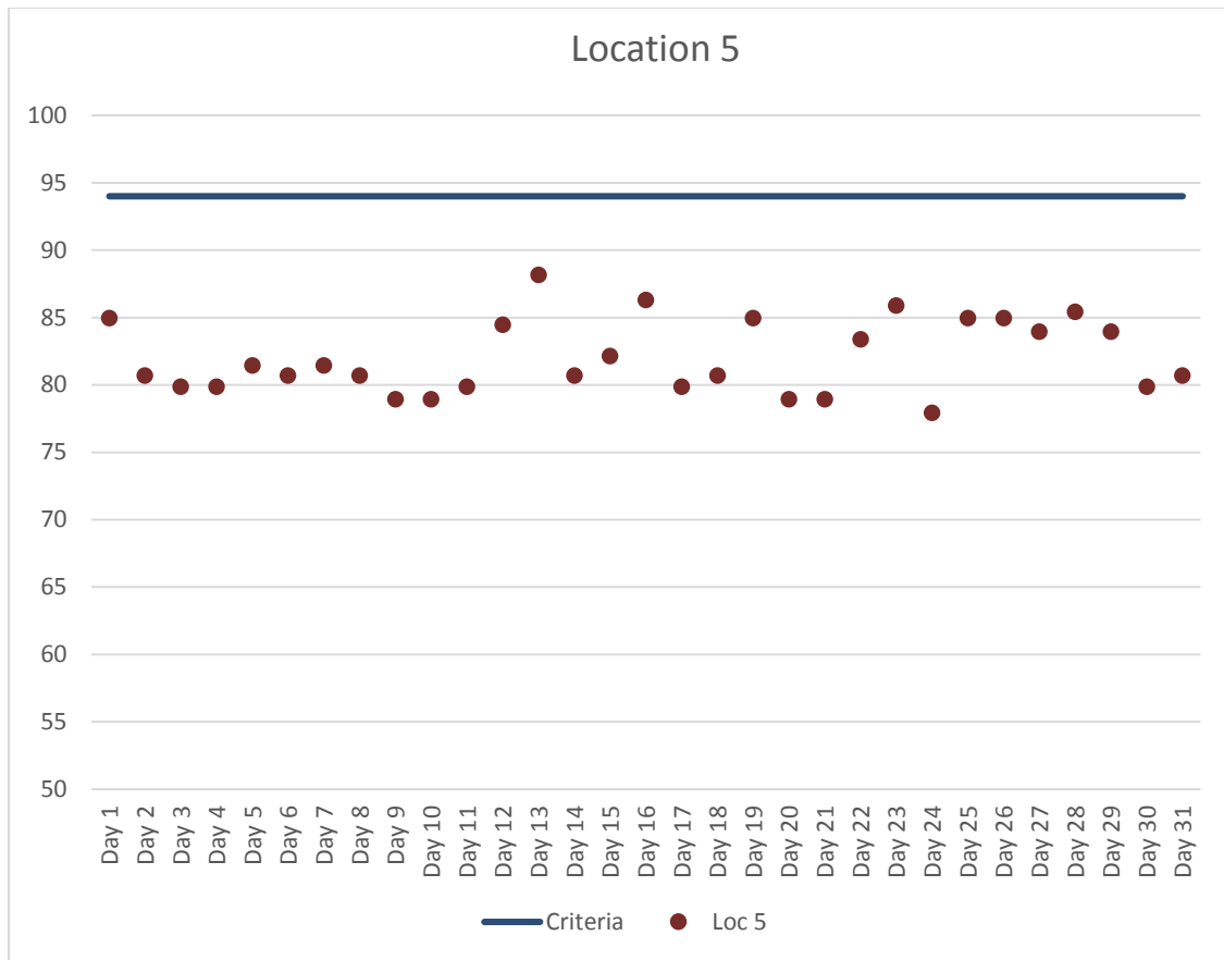
Figure 6. Location 5 Maximum Daily Construction Vibration Monitoring Data (VdB) – March 2018
