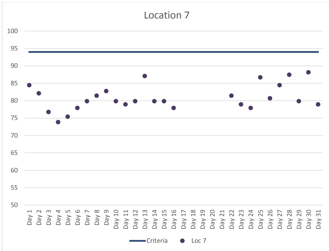
Figure 8. Location 7 Maximum Daily Construction Vibration Monitoring Data (VdB) –March 2018
