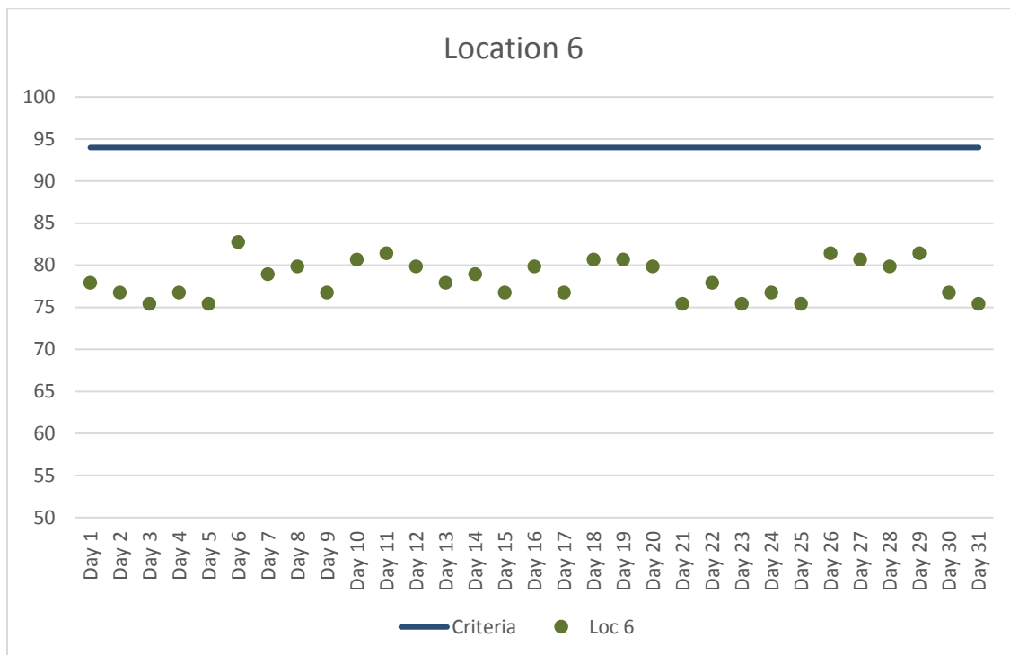
Figure 7. Location 6 Maximum Daily Construction Vibration Monitoring Data (VdB) – March 2018
