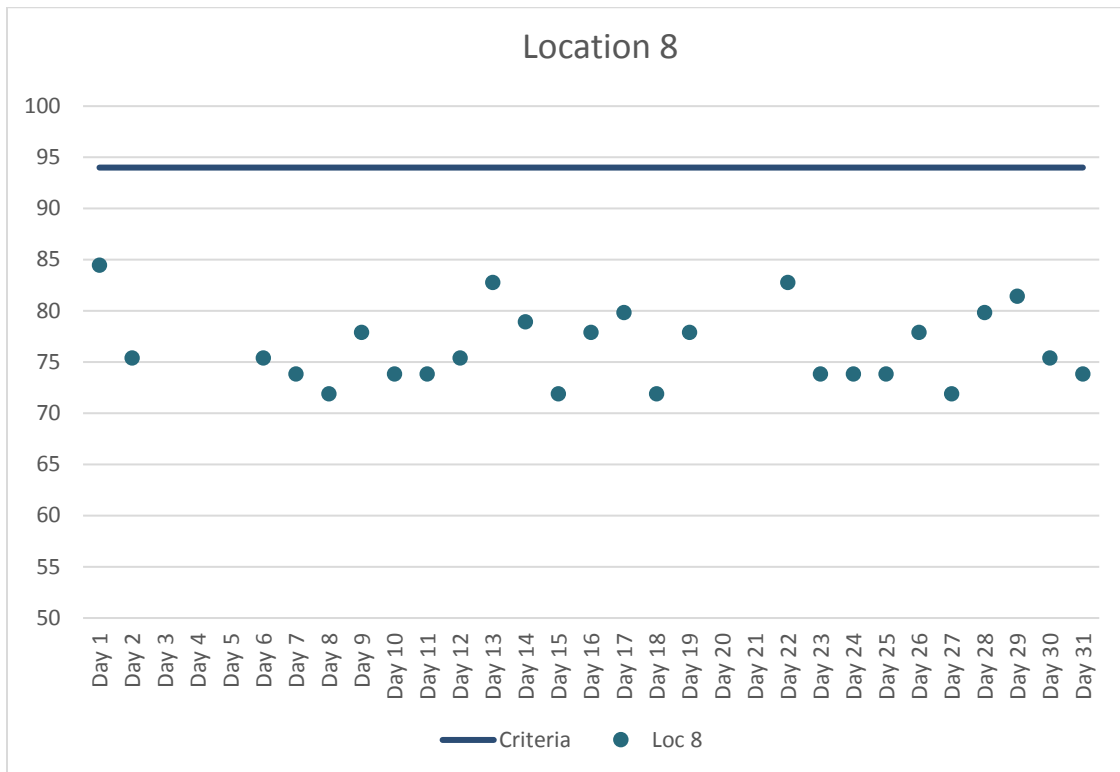
Figure 9. Location 8 Maximum Daily Construction Vibration Monitoring Data (VdB) –March 2018
