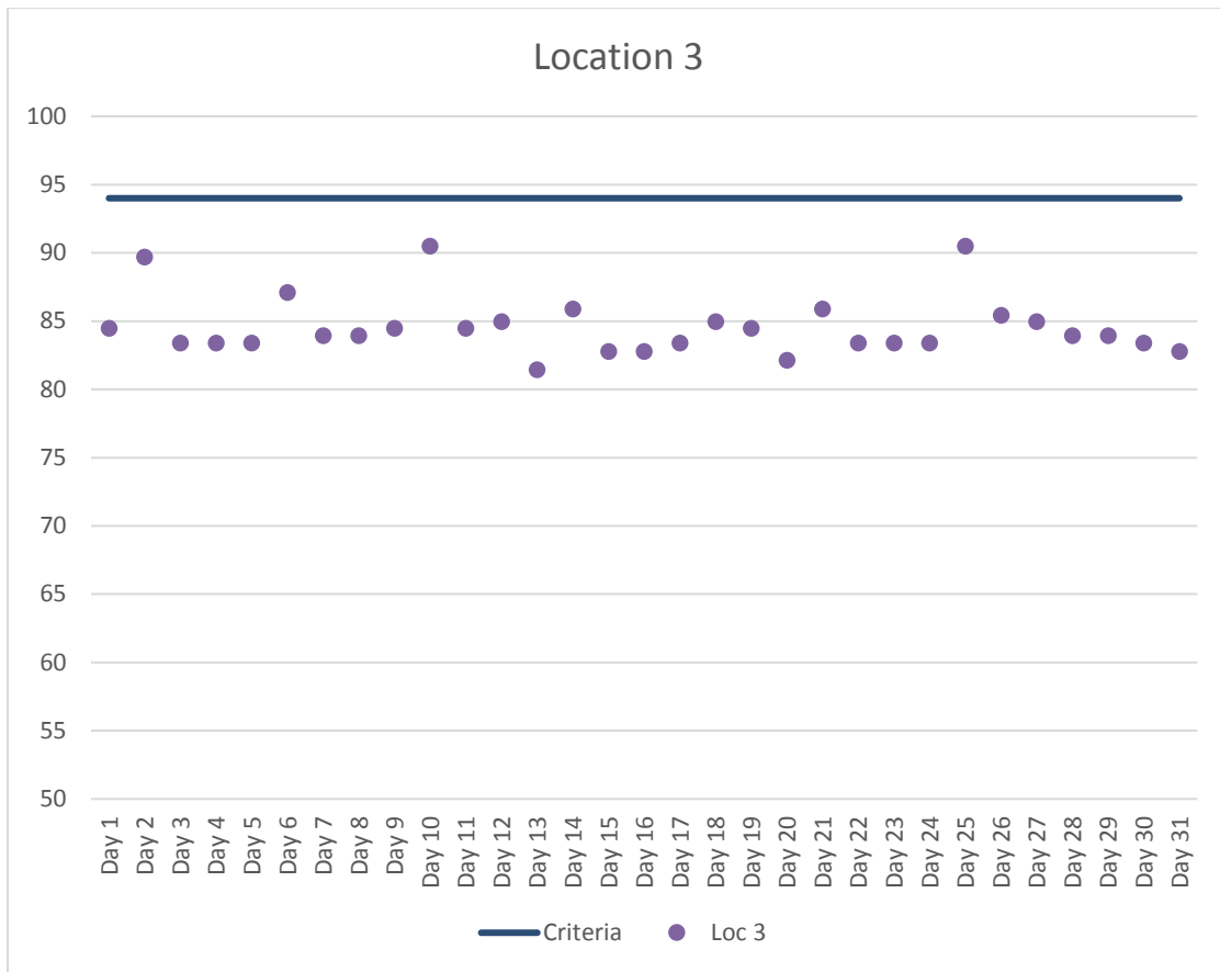
Figure 4. Location 3 Maximum Daily Construction Vibration Monitoring Data (VdB) –March 2018
