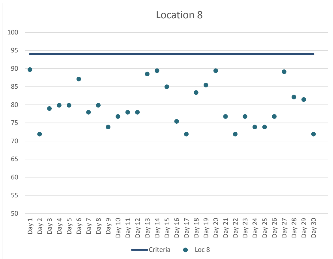
Figure 9. Location 8 Maximum Daily Construction Vibration Monitoring Data (VdB) – June 2018
