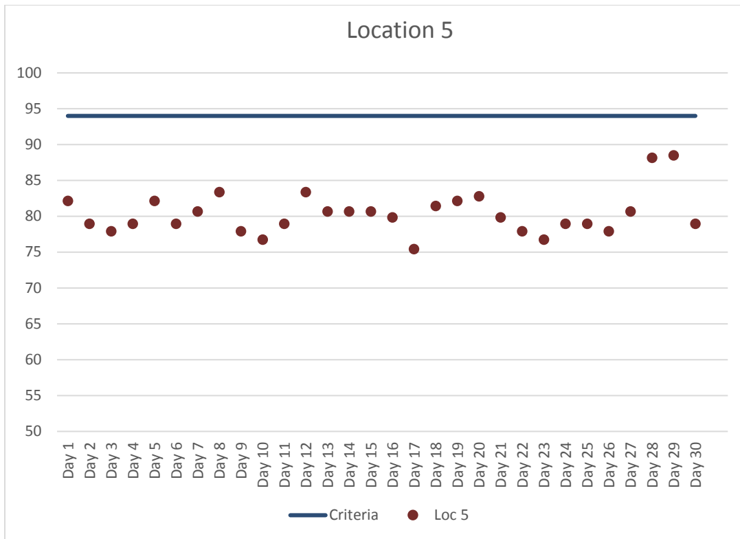
Figure 6. Location 5 Maximum Daily Construction Vibration Monitoring Data (VdB) – June 2018
