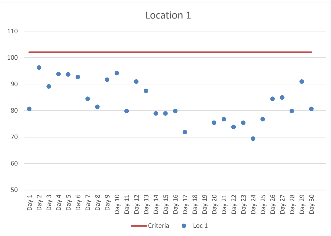
Figure 2. Location 1 Maximum Daily Construction Vibration Monitoring Data (VdB) – June 2018
