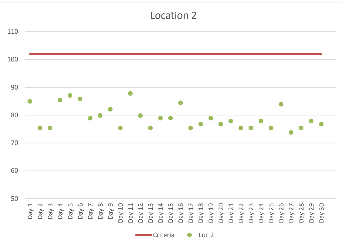
Figure 3. Location 2 Maximum Daily Construction Vibration Monitoring Data (VdB) – June 2018
