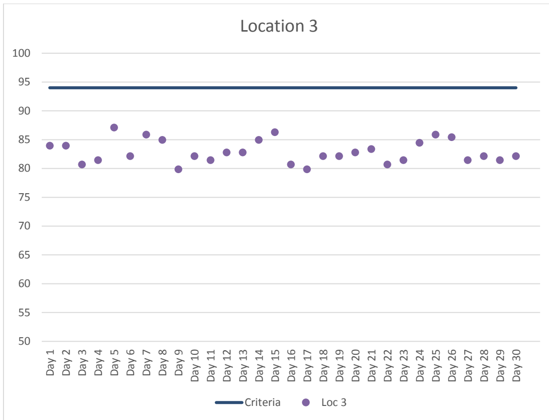
Figure 4. Location 3 Maximum Daily Construction Vibration Monitoring Data (VdB) – June 2018
