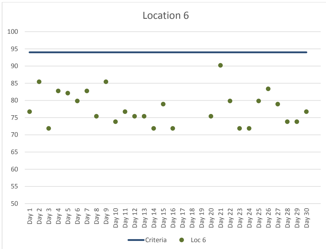
Figure 7. Location 6 Maximum Daily Construction Vibration Monitoring Data (VdB) – June 2018
