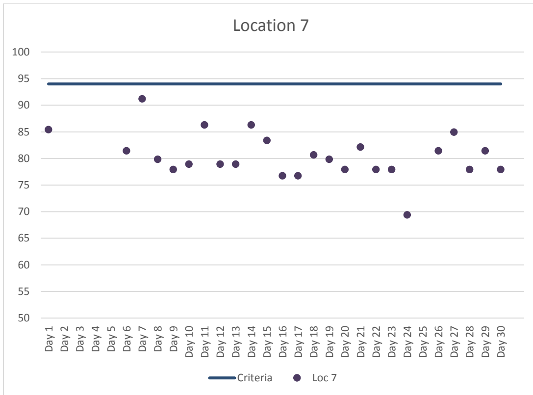
Figure 8. Location 7 Maximum Daily Construction Vibration Monitoring Data (VdB) – June 2018
