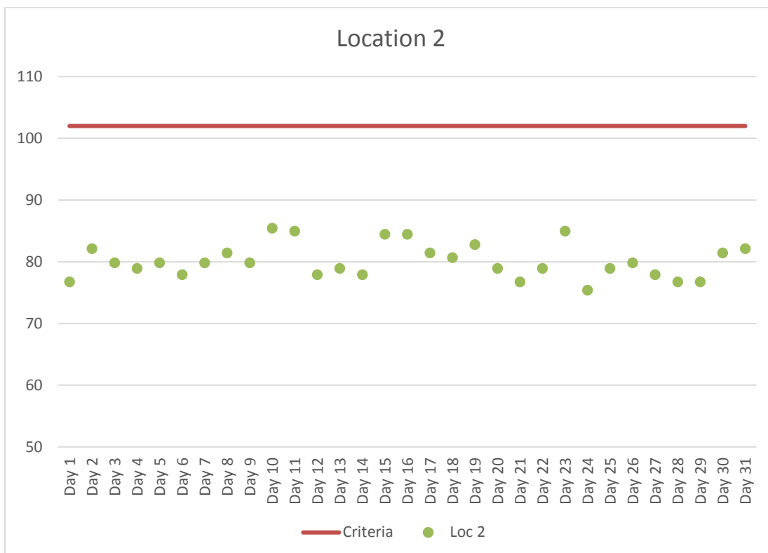
Figure 3. Location 2 Maximum Daily Construction Vibration Monitoring Data (VdB) – January 2018
