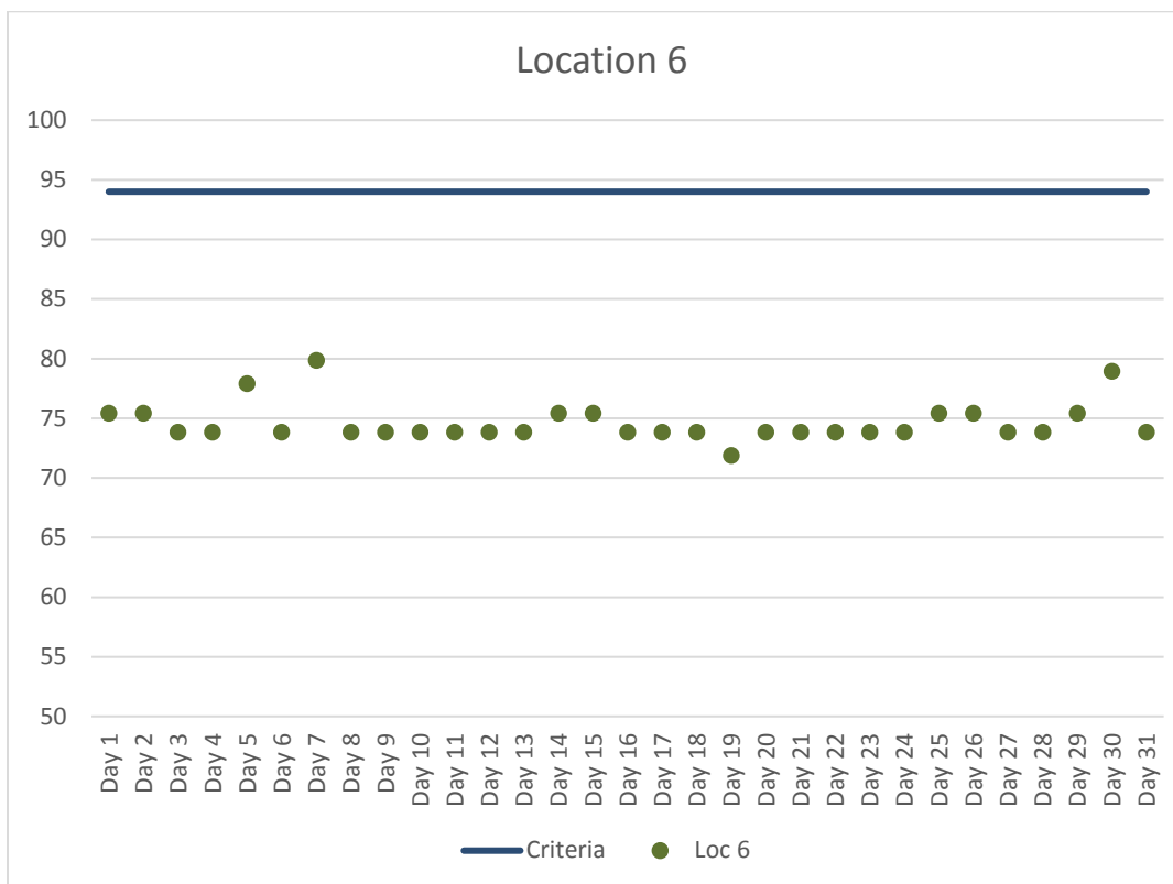
Figure 7. Location 6 Maximum Daily Construction Vibration Monitoring Data (VdB) – January 2018
