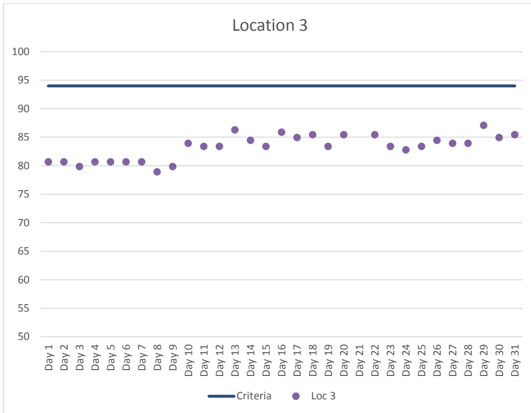
Figure 4. Location 3 Maximum Daily Construction Vibration Monitoring Data (VdB) – January 2018
