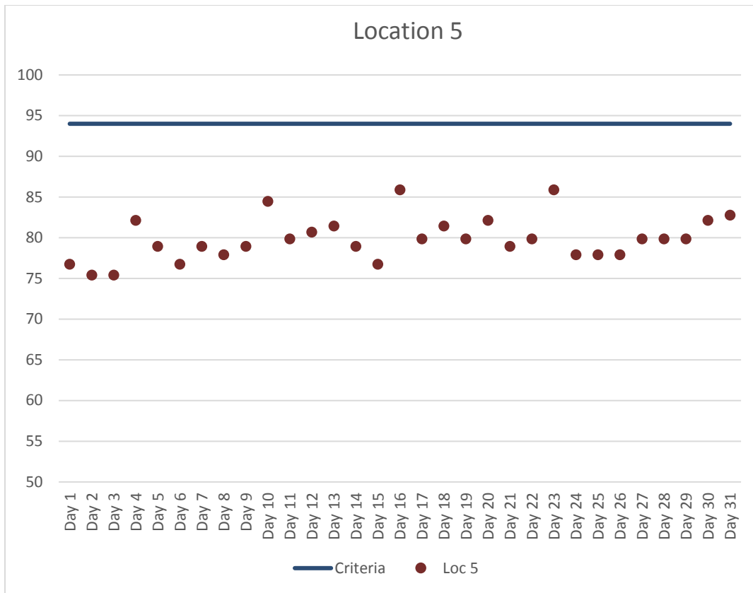
Figure 6. Location 5 Maximum Daily Construction Vibration Monitoring Data (VdB) – January 2018
