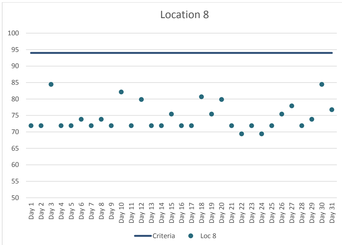
Figure 9. Location 8 Maximum Daily Construction Vibration Monitoring Data (VdB) – January 2018
