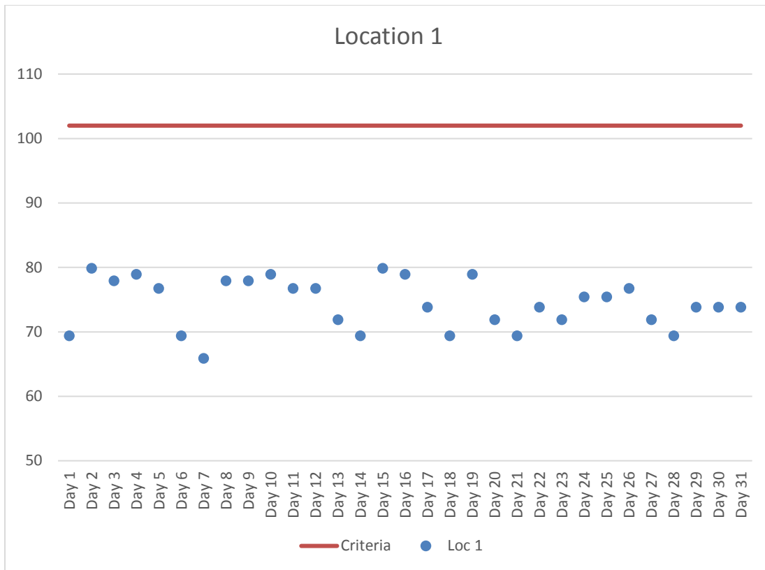
Figure 2. Location 1 Maximum Daily Construction Vibration Monitoring Data (VdB) – January 2018
