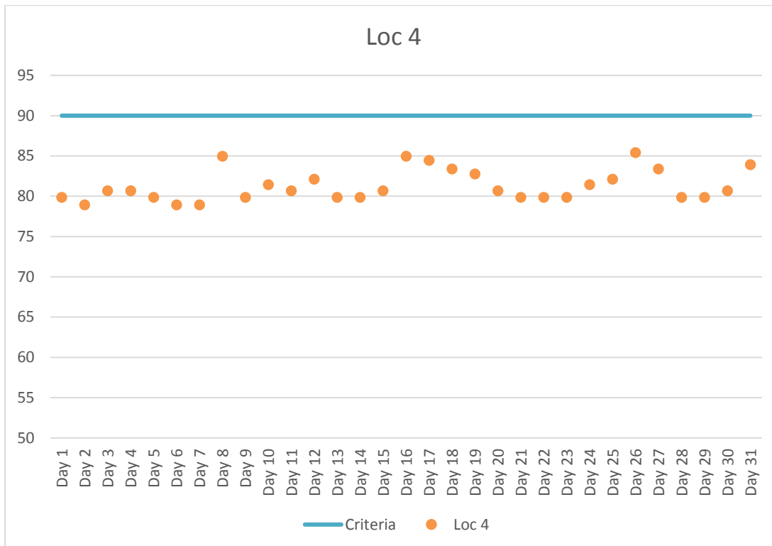
Figure 5. Location 4 Maximum Daily Construction Vibration Monitoring Data (VdB) – January 2018
