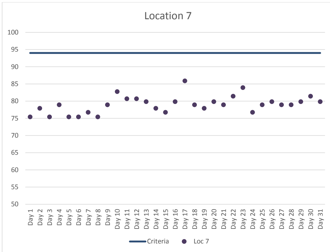
Figure 8. Location 7 Maximum Daily Construction Vibration Monitoring Data (VdB) – January 2018
