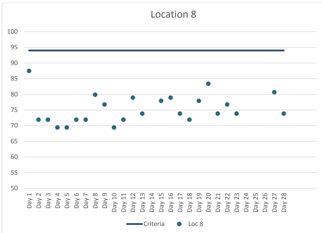
Figure 9. Location 8 Maximum Daily Construction Vibration Monitoring Data (VdB) – February 2018
