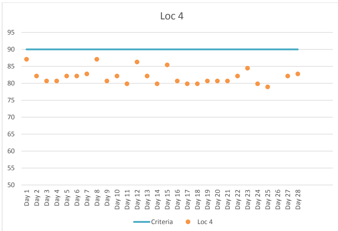
Figure 5. Location 4 Maximum Daily Construction Vibration Monitoring Data (VdB) – February 2018
