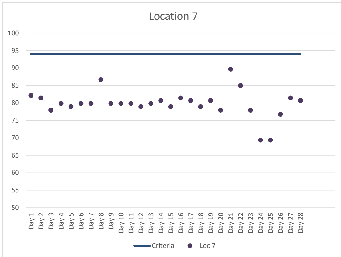
Figure 8. Location 7 Maximum Daily Construction Vibration Monitoring Data (VdB) – February 2018
