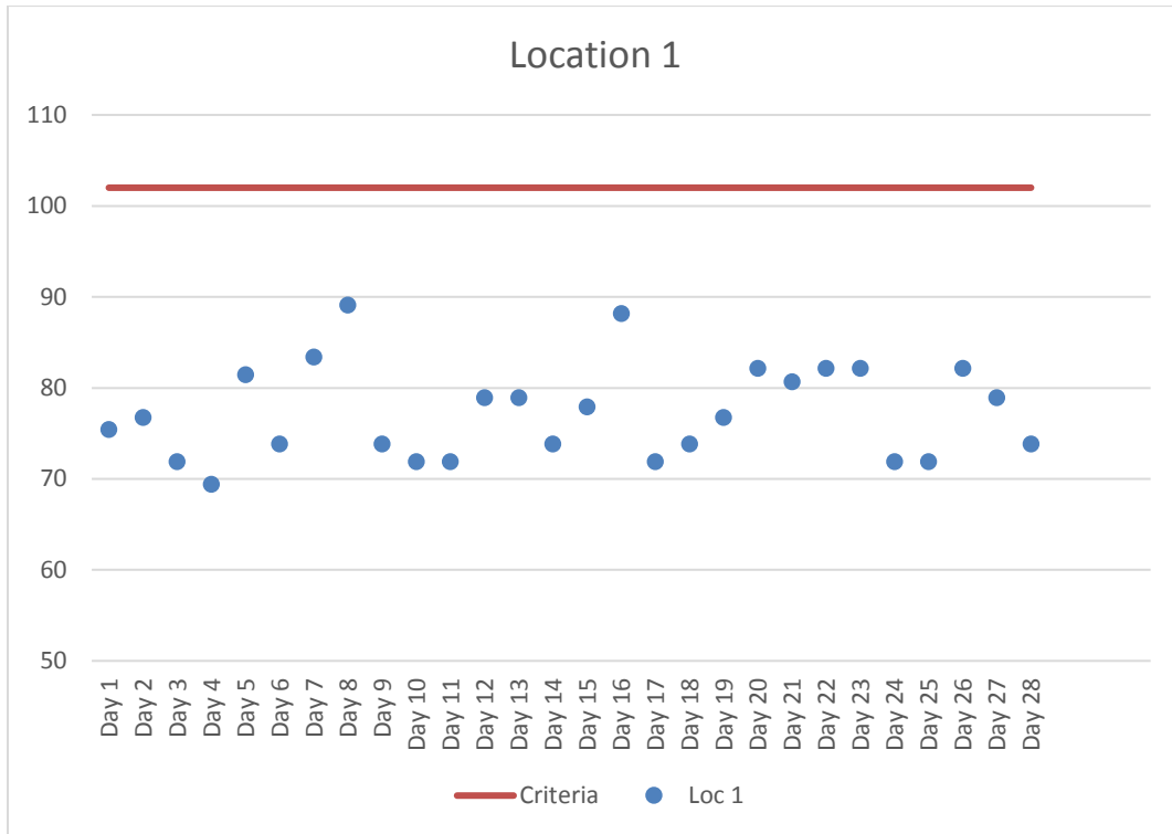
Figure 2. Location 1 Maximum Daily Construction Vibration Monitoring Data (VdB) – February 2018
