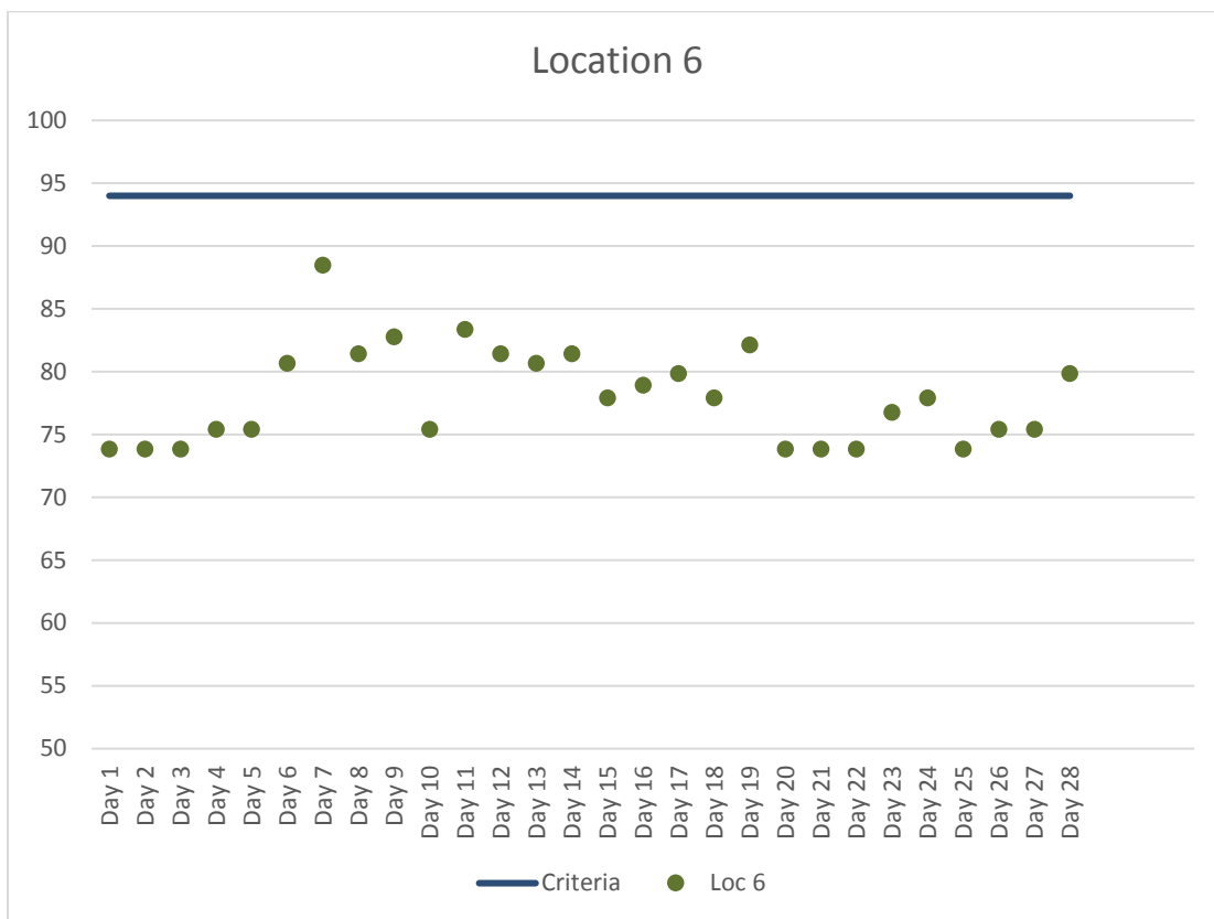
Figure 7. Location 6 Maximum Daily Construction Vibration Monitoring Data (VdB) – February 2018
