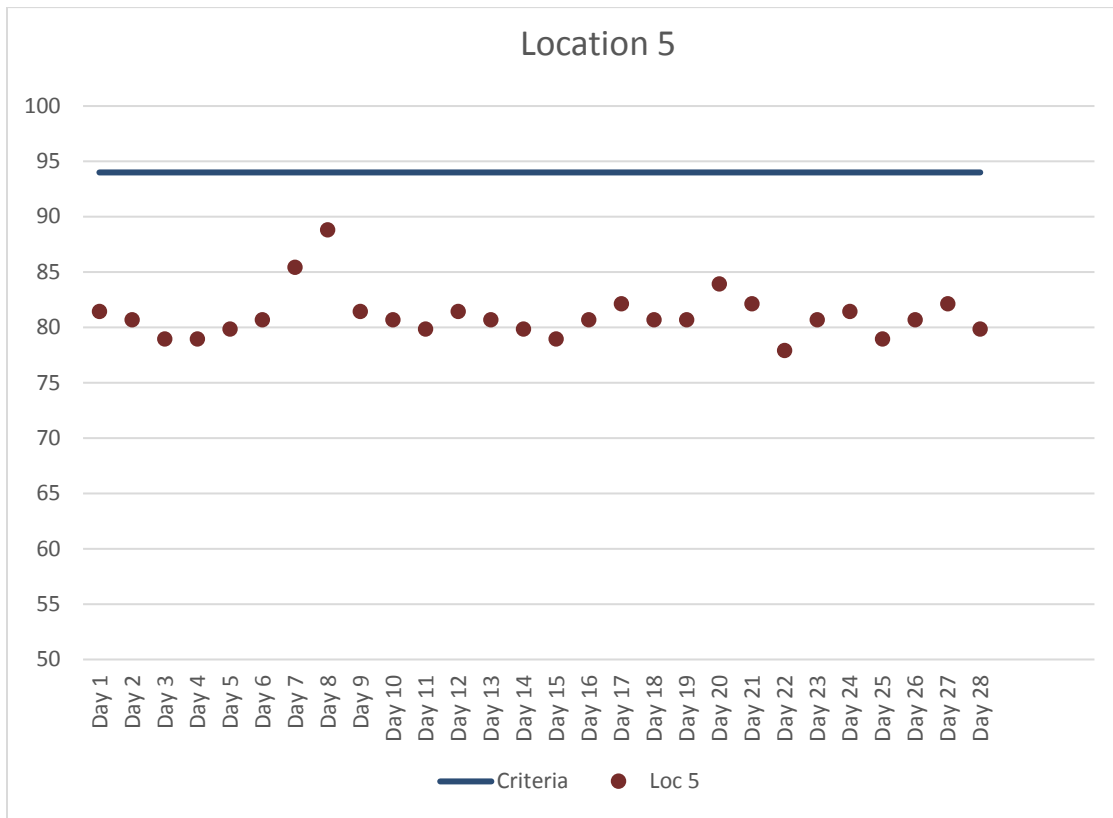
Figure 6. Location 5 Maximum Daily Construction Vibration Monitoring Data (VdB) – February 2018
