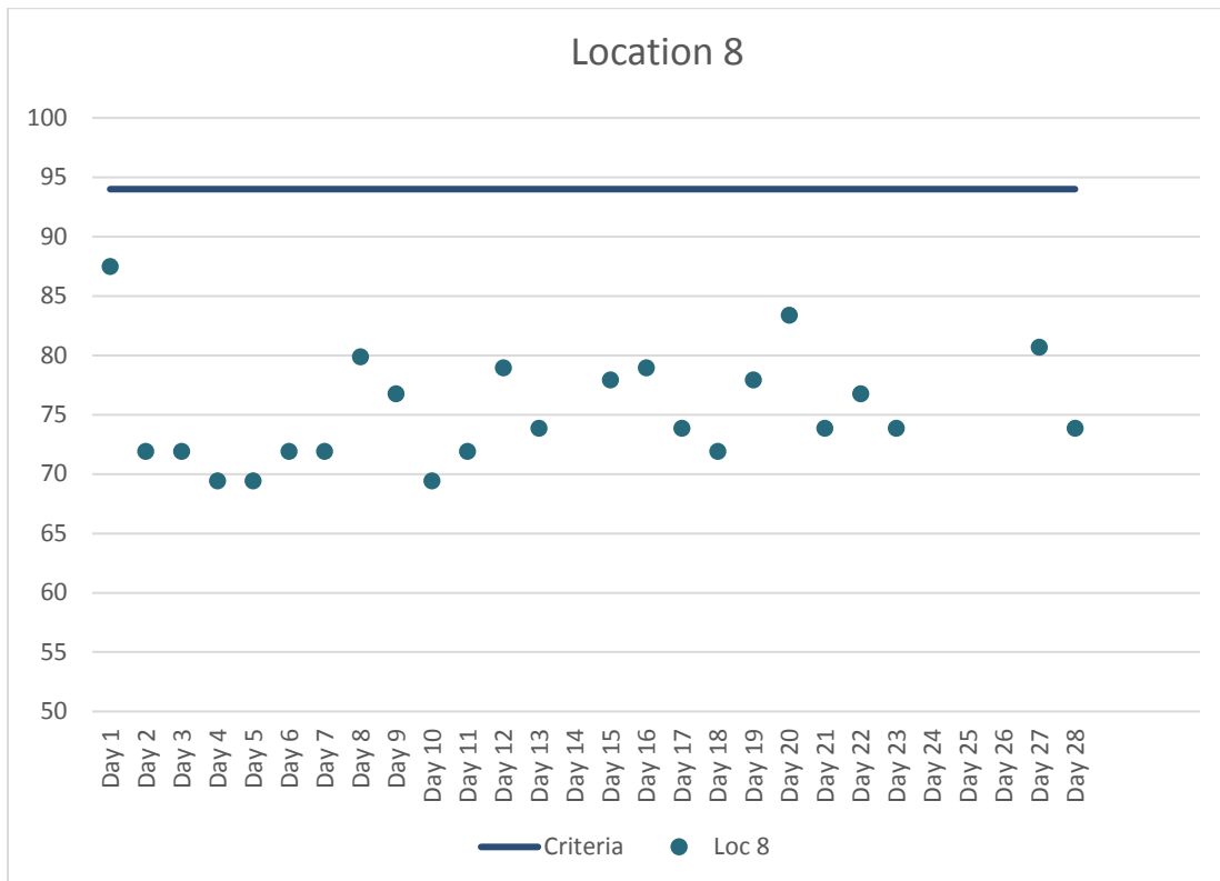
Figure 9. Location 8 Maximum Daily Construction Vibration Monitoring Data (VdB) – February 2018
