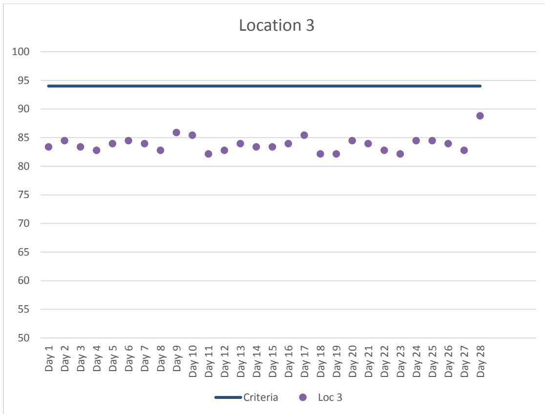
Figure 4. Location 3 Maximum Daily Construction Vibration Monitoring Data (VdB) – February 2018
