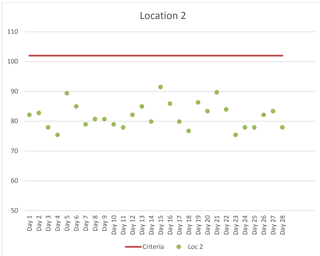
Figure 3. Location 2 Maximum Daily Construction Vibration Monitoring Data (VdB) – February 2018
