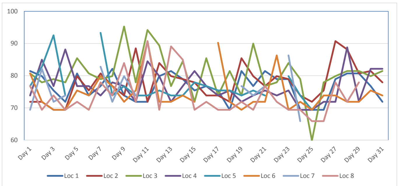
Figure 2. Summary of Construction Vibration Monitoring Data (VdB) – December 2016
