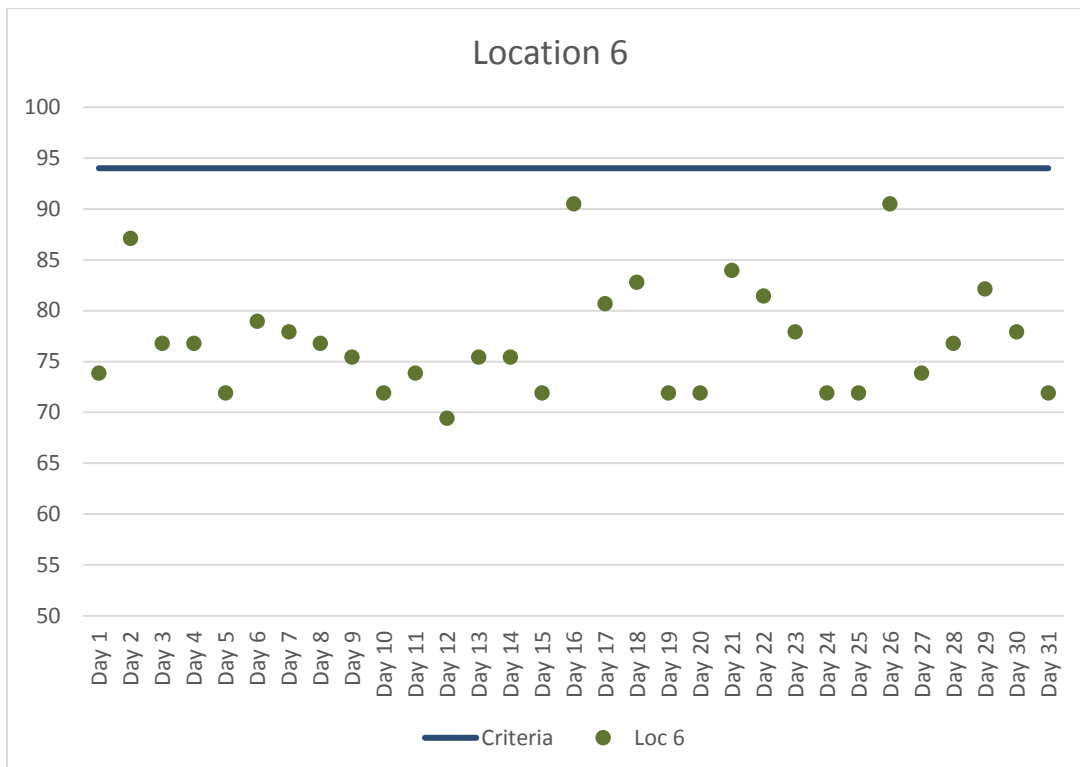
Figure 7. Location 6 Maximum Daily Construction Vibration Monitoring Data (VdB) – August 2018
