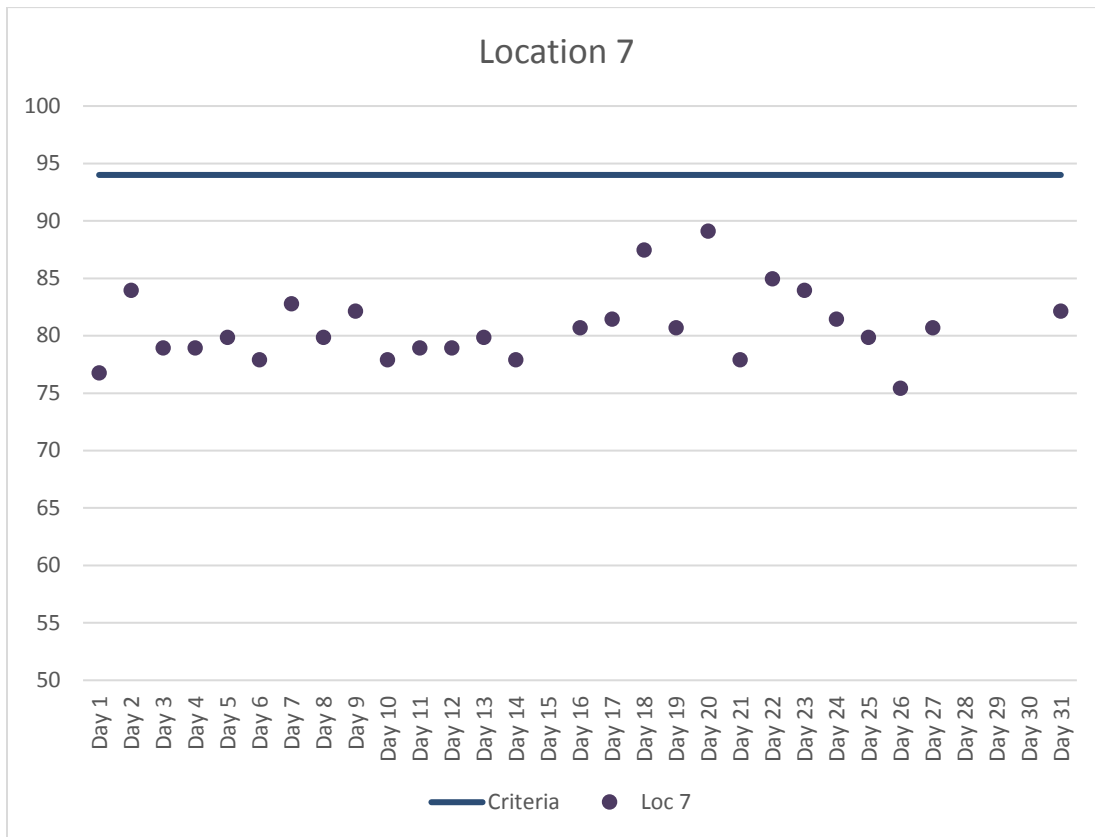
Figure 8. Location 7 Maximum Daily Construction Vibration Monitoring Data (VdB) – August 2018
