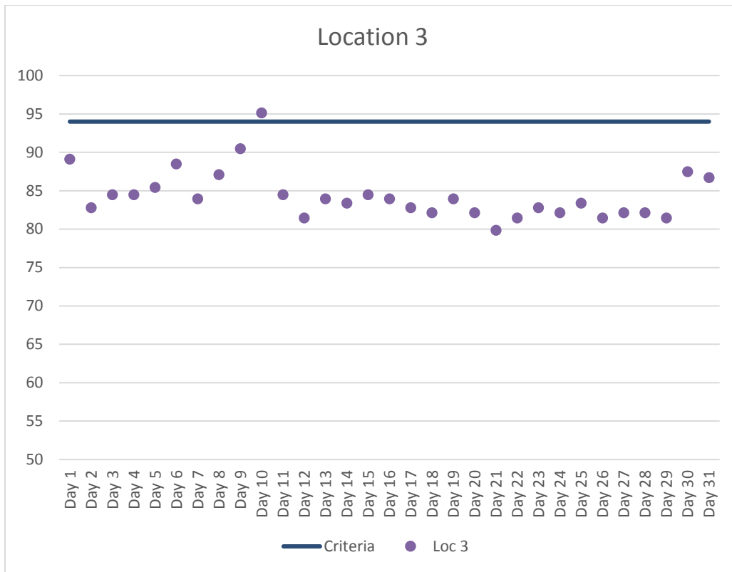
Figure 4. Location 3 Maximum Daily Construction Vibration Monitoring Data (VdB) – August 2018
