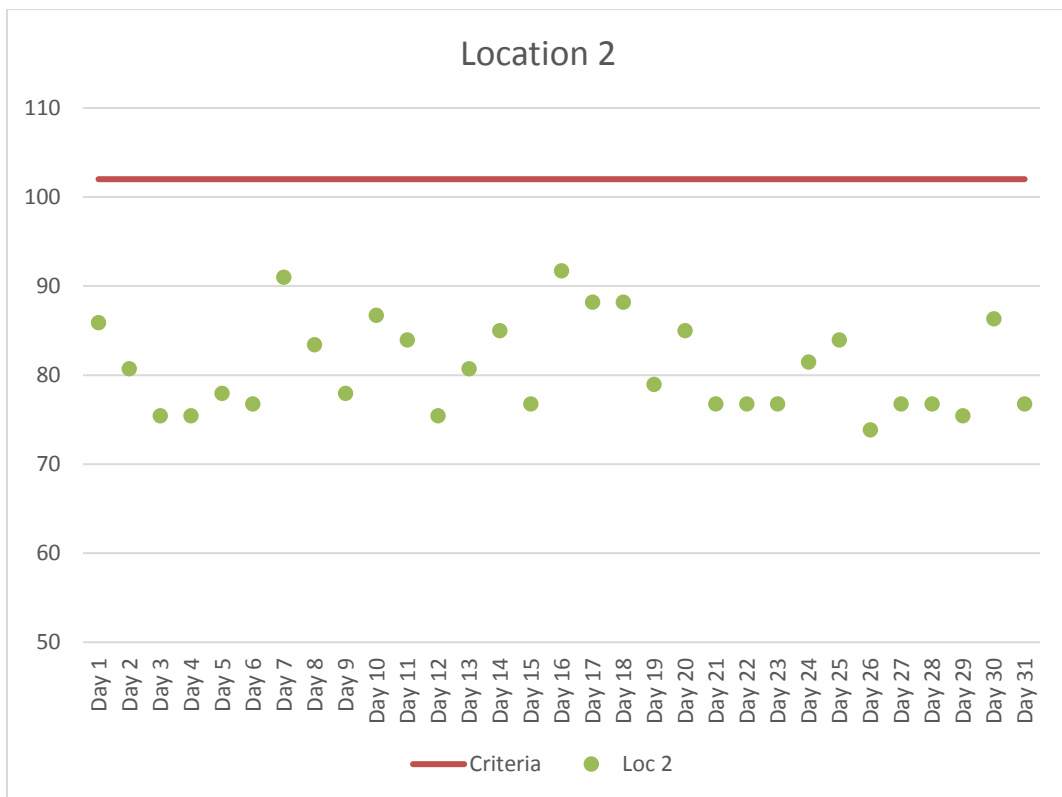
Figure 3. Location 2 Maximum Daily Construction Vibration Monitoring Data (VdB) – August 2018
