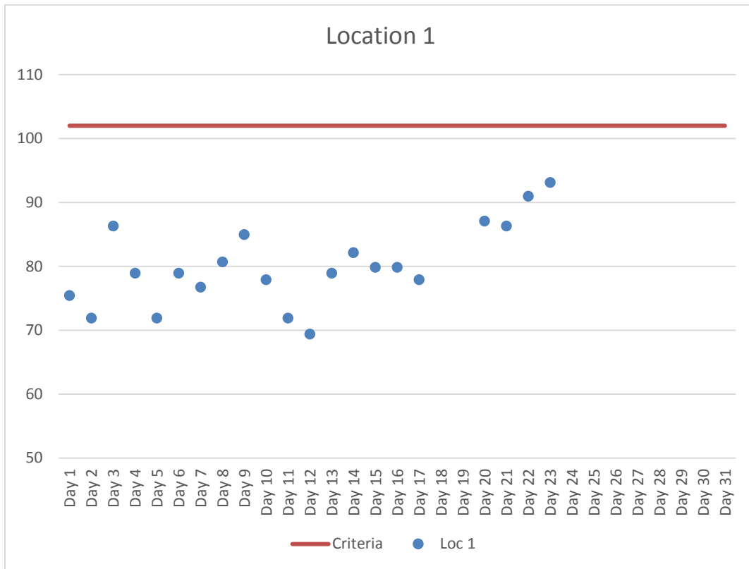
Figure 2. Location 1 Maximum Daily Construction Vibration Monitoring Data (VdB) – August 2018
