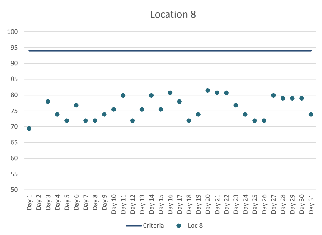
Figure 9. Location 8 Maximum Daily Construction Vibration Monitoring Data (VdB) – August 2018
