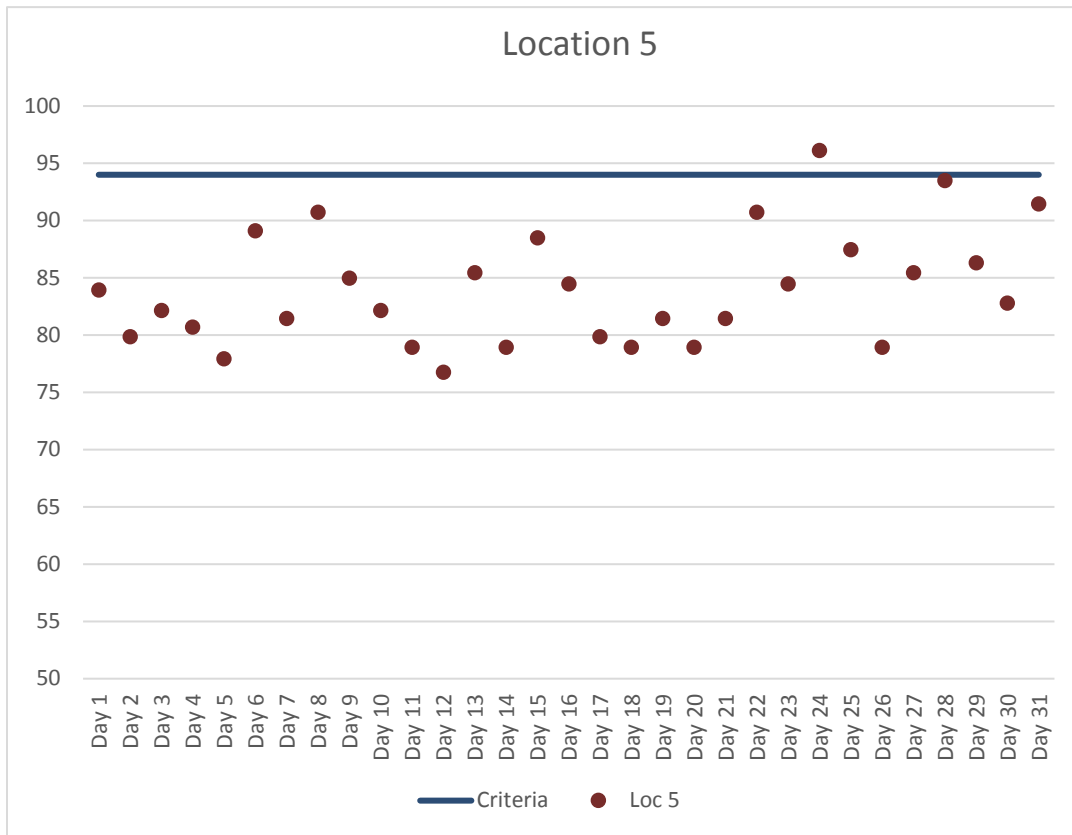
Figure 6. Location 5 Maximum Daily Construction Vibration Monitoring Data (VdB) – August 2018
