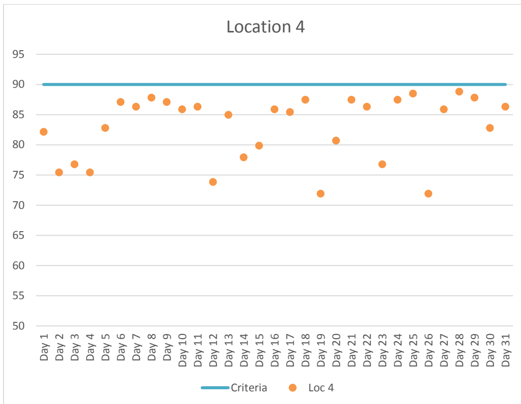
Figure 5. Location 4 Maximum Daily Construction Vibration Monitoring Data (VdB) – August 2018
