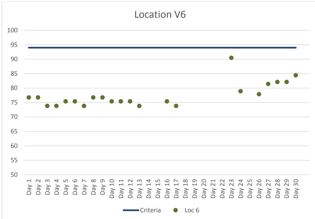
Figure 7. Location V6 Maximum Daily Construction Vibration Monitoring Data (VdB) – April 2018
