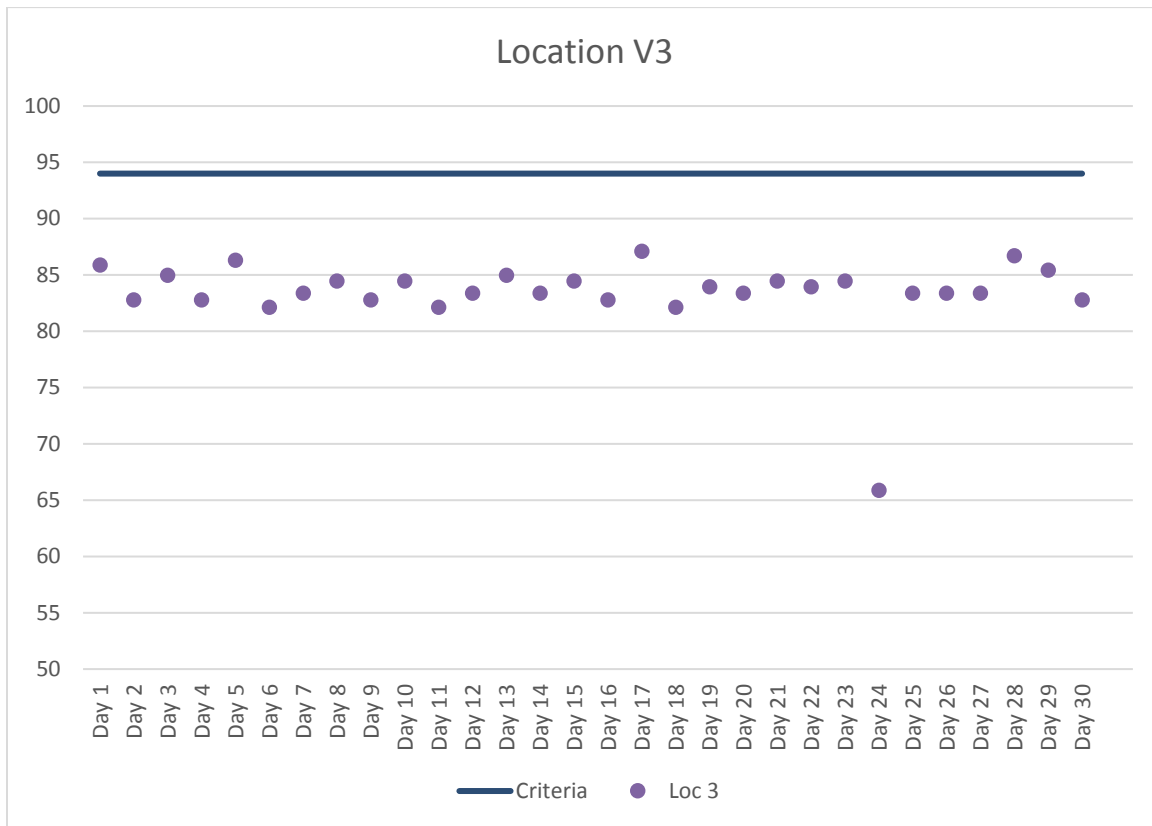
Figure 4. Location V3 Maximum Daily Construction Vibration Monitoring Data (VdB) – April 2018
