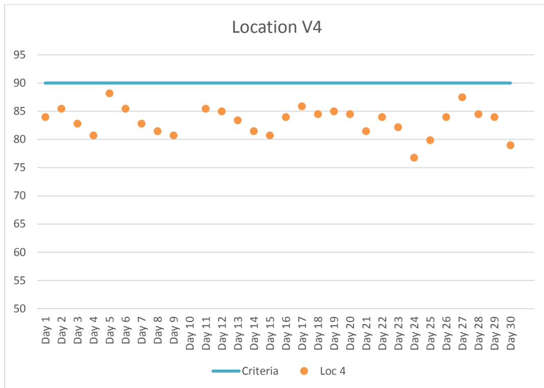
Figure 5. Location V4 Maximum Daily Construction Vibration Monitoring Data (VdB) – April 2018
