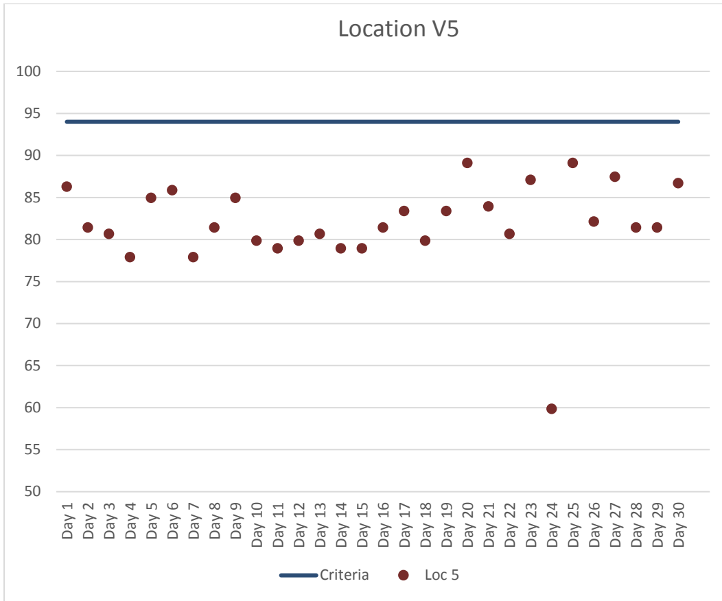
Figure 6. Location V5 Maximum Daily Construction Vibration Monitoring Data (VdB) – April 2018
