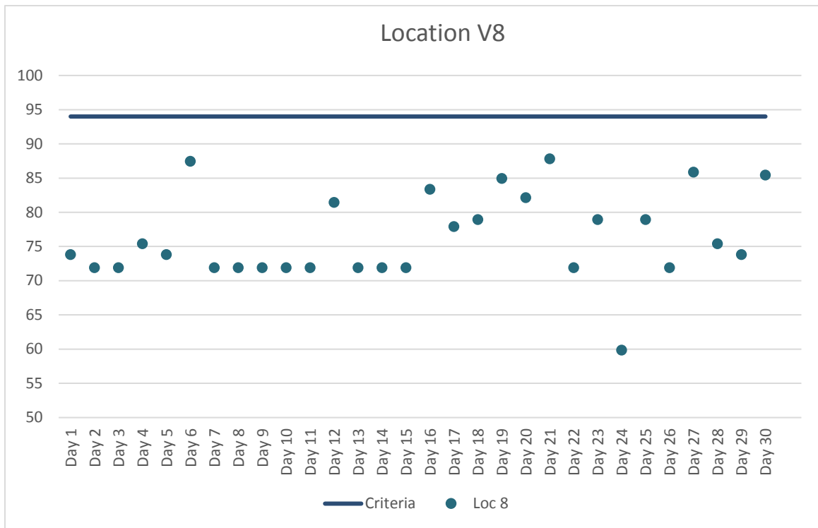
Figure 9. Location V8 Maximum Daily Construction Vibration Monitoring Data (VdB) – April 2018
