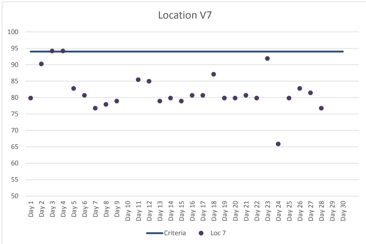
Figure 8. Location V7 Maximum Daily Construction Vibration Monitoring Data (VdB) – April 2018
