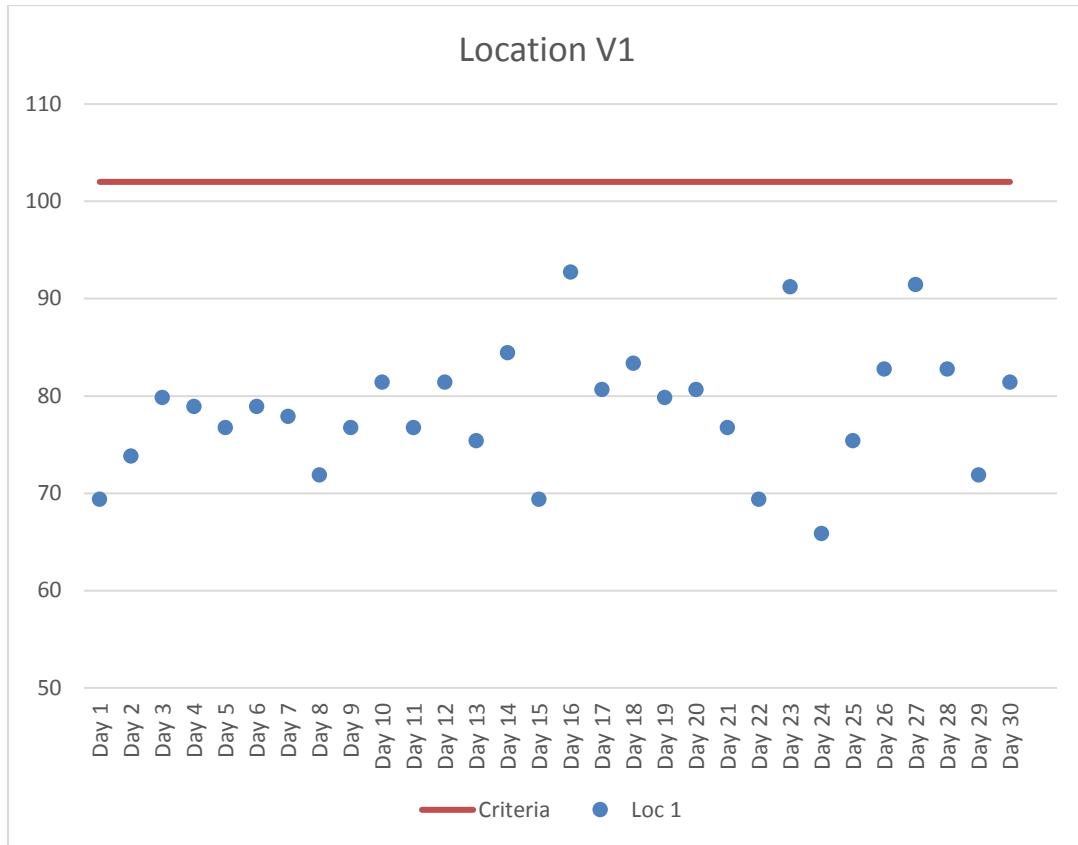
Figure 2. Location V1 Maximum Daily Construction Vibration Monitoring Data (VdB) – April 2018
