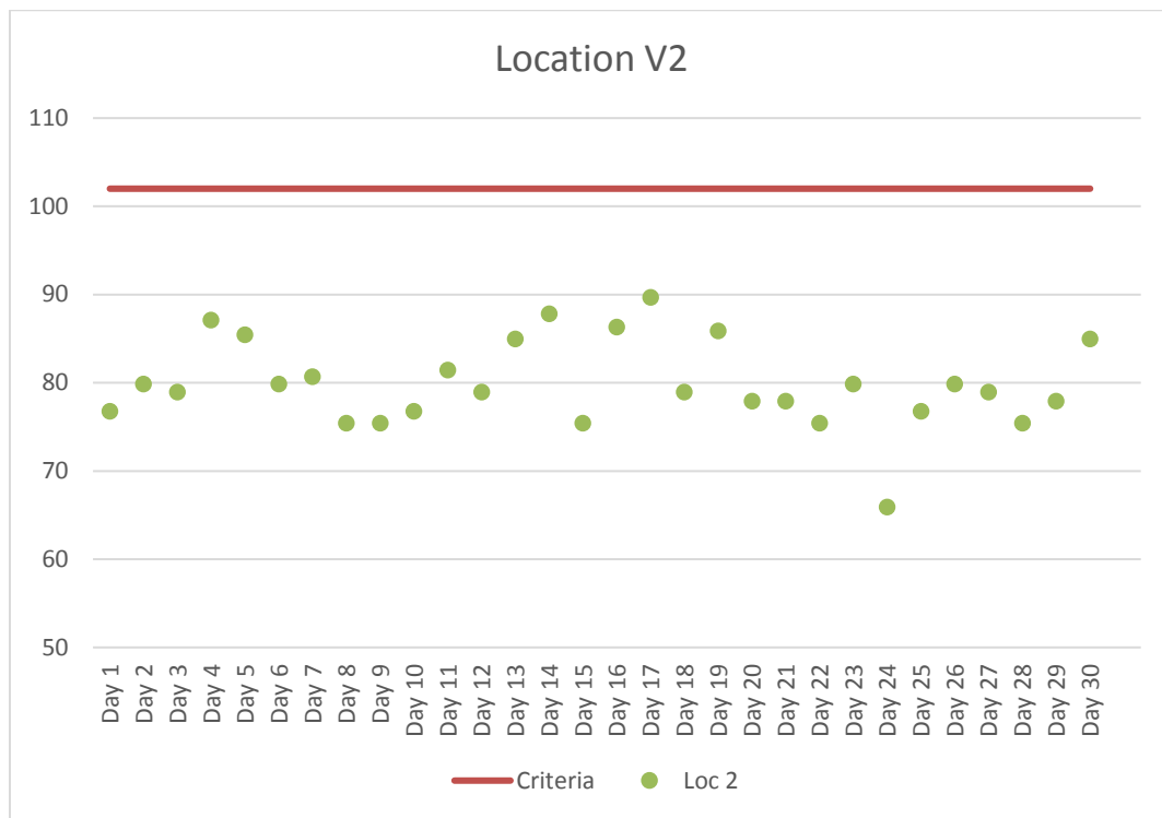
Figure 3. Location V2 Maximum Daily Construction Vibration Monitoring Data (VdB) – April 2018
