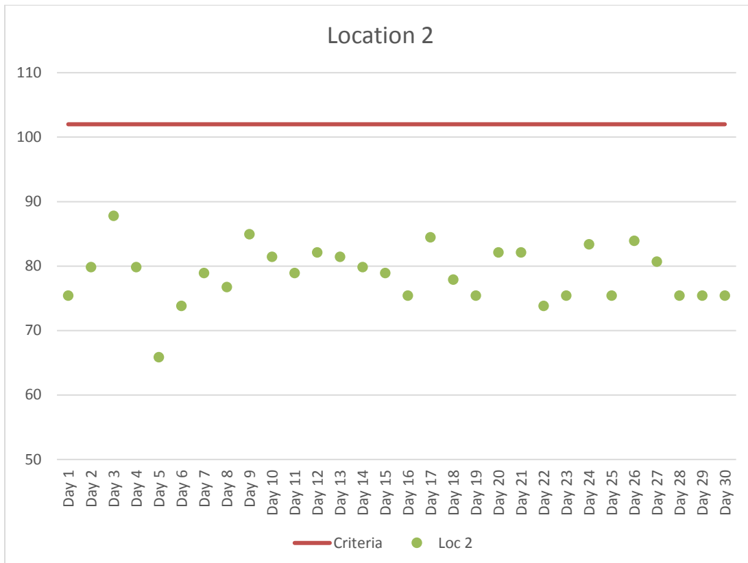
Figure 3. Location 2 Maximum Daily Construction Vibration Monitoring Data (VdB) – April 2017
