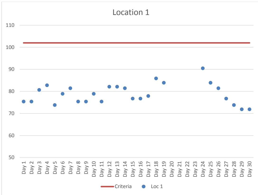
Figure 2. Location 1 Maximum Daily Construction Vibration Monitoring Data (VdB) – April 2017
