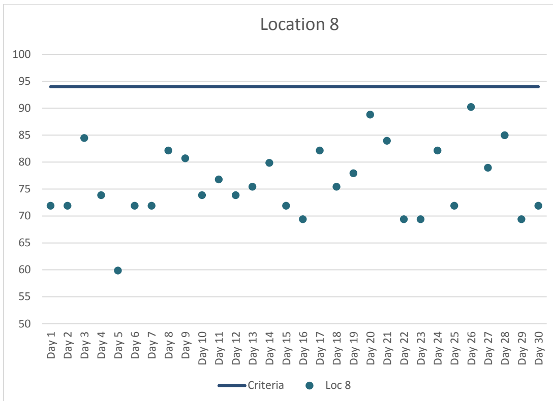
Figure 9. Location 8 Maximum Daily Construction Vibration Monitoring Data (VdB) – April 2017
