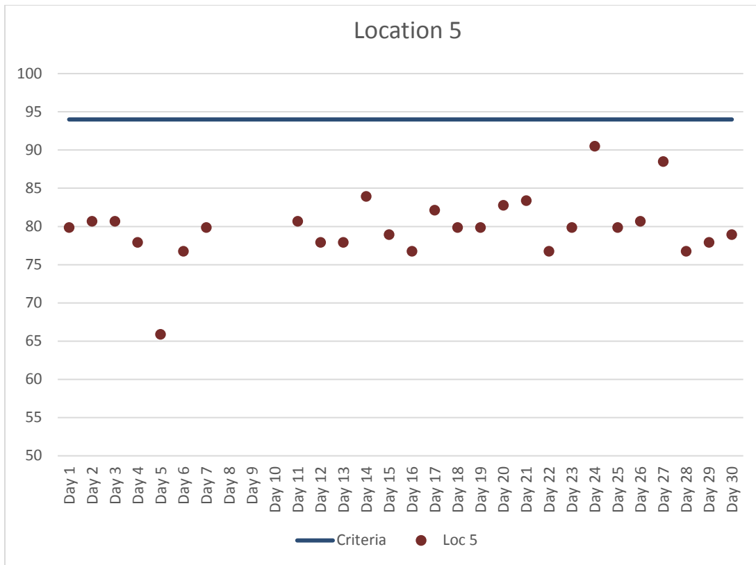
Figure 6. Location 5 Maximum Daily Construction Vibration Monitoring Data (VdB) – April 2017
