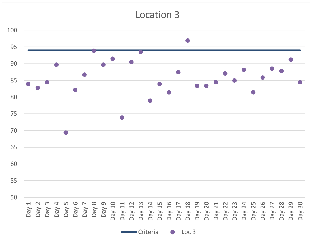
Figure 4. Location 3 Maximum Daily Construction Vibration Monitoring Data (VdB) – April 2017
