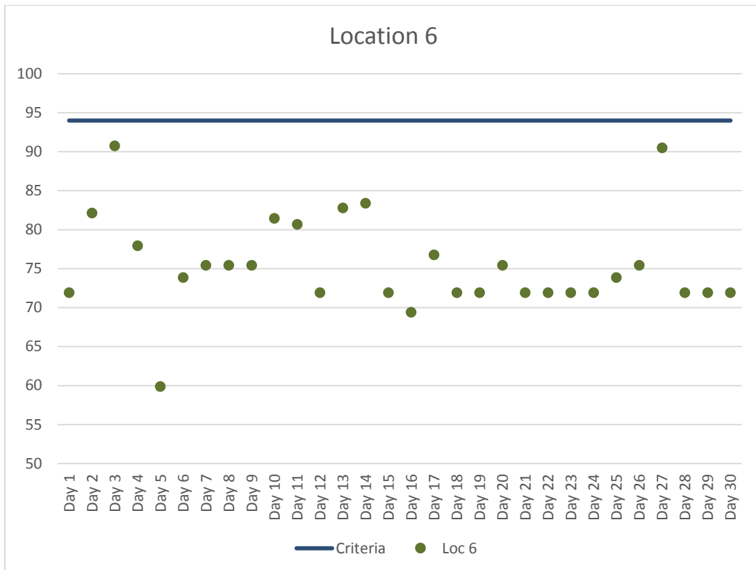
Figure 7. Location 6 Maximum Daily Construction Vibration Monitoring Data (VdB) – April 2017
