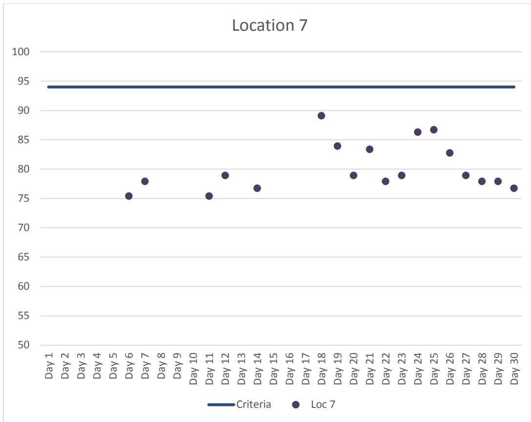
Figure 8. Location 7 Maximum Daily Construction Vibration Monitoring Data (VdB) – April 2017
