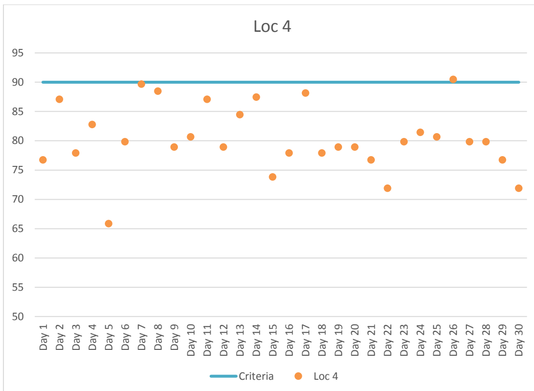
Figure 5. Location 4 Maximum Daily Construction Vibration Monitoring Data (VdB) – April 2017
