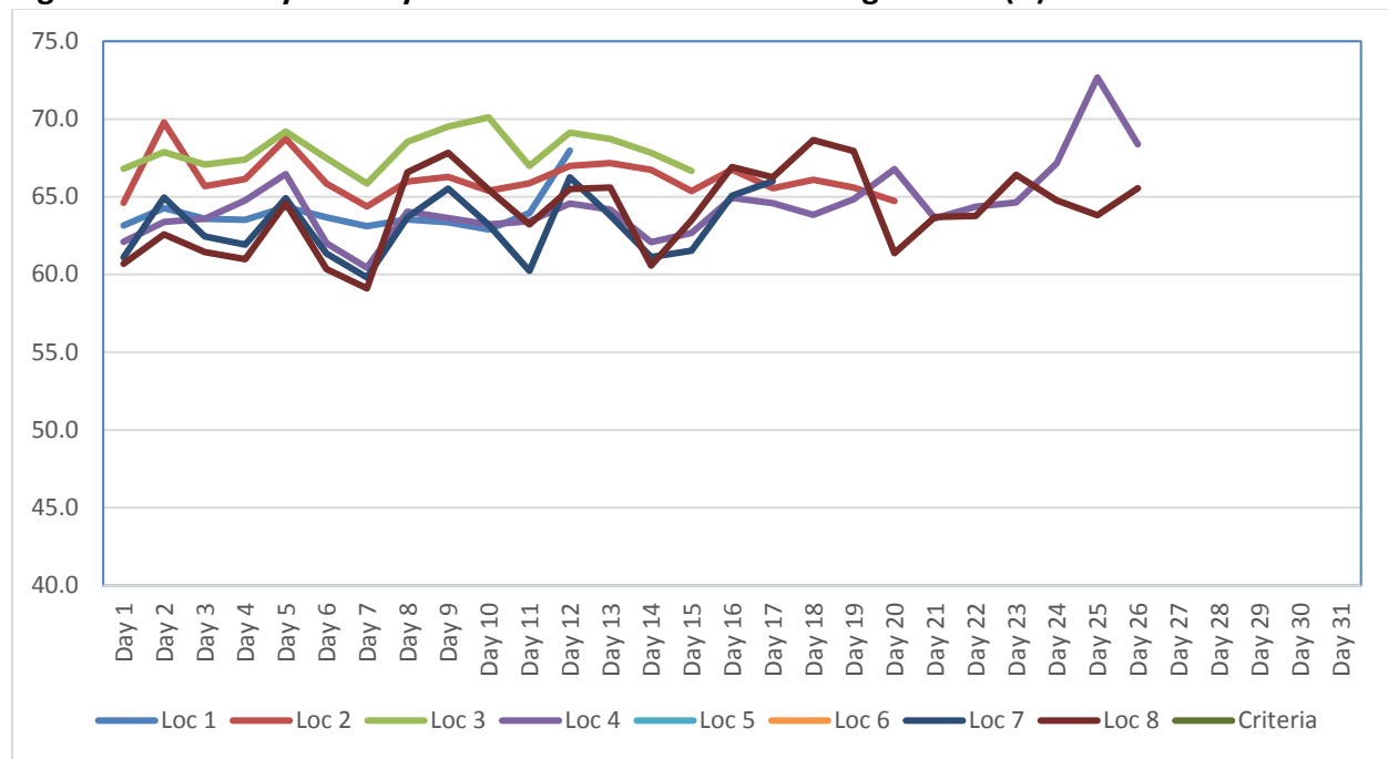
Figure 2. Summary of Daily Construction Noise Monitoring Data dB(A) – October 2018
