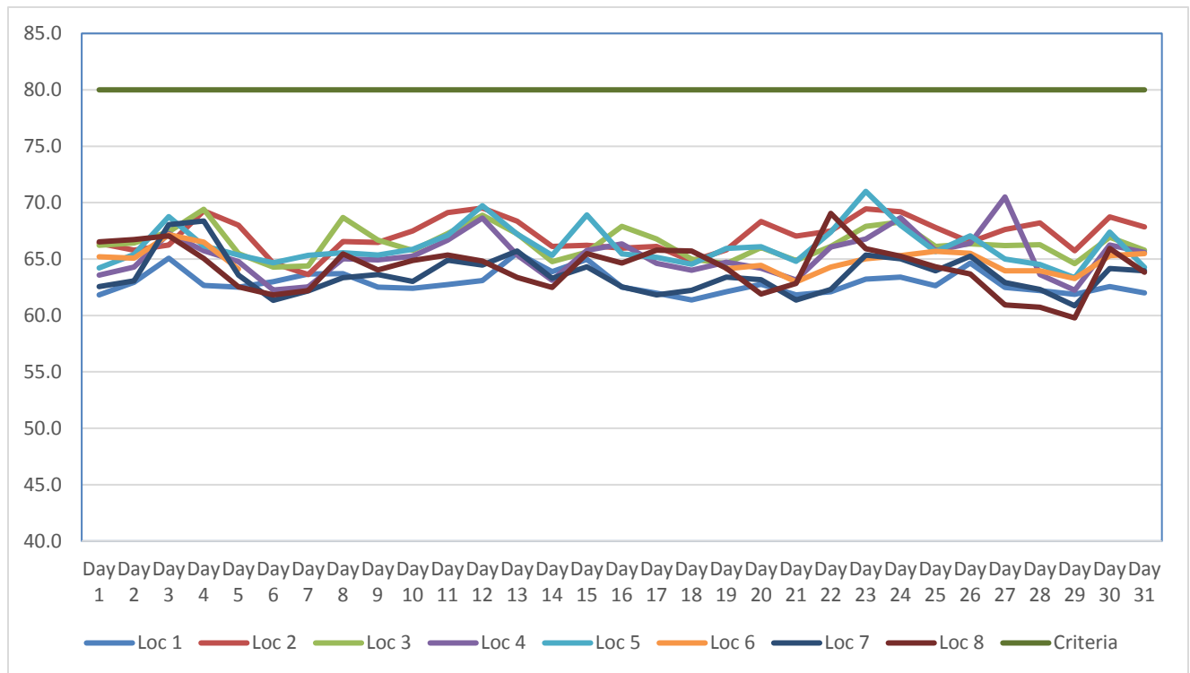
Figure 2. Summary of Daily Construction Noise Monitoring Data dB(A) – May 2017
