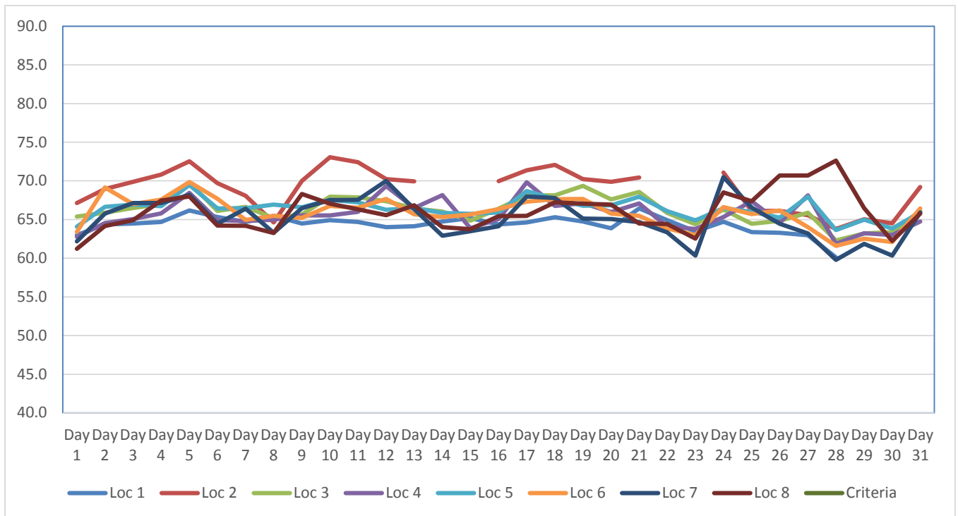
Figure 2. Summary of Daily Construction Noise Monitoring Data dB(A) – May 2016
