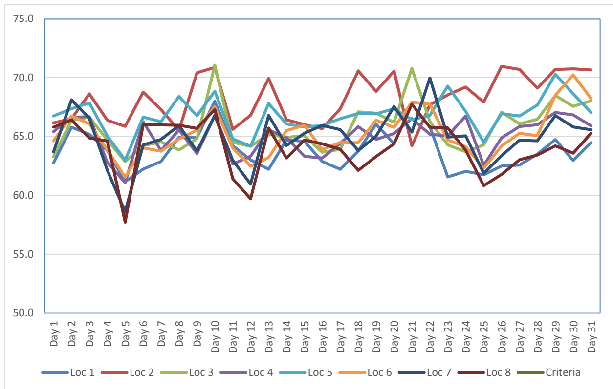
Figure 2. Summary of Daily Construction Noise Monitoring Data dB(A) – March 2017
