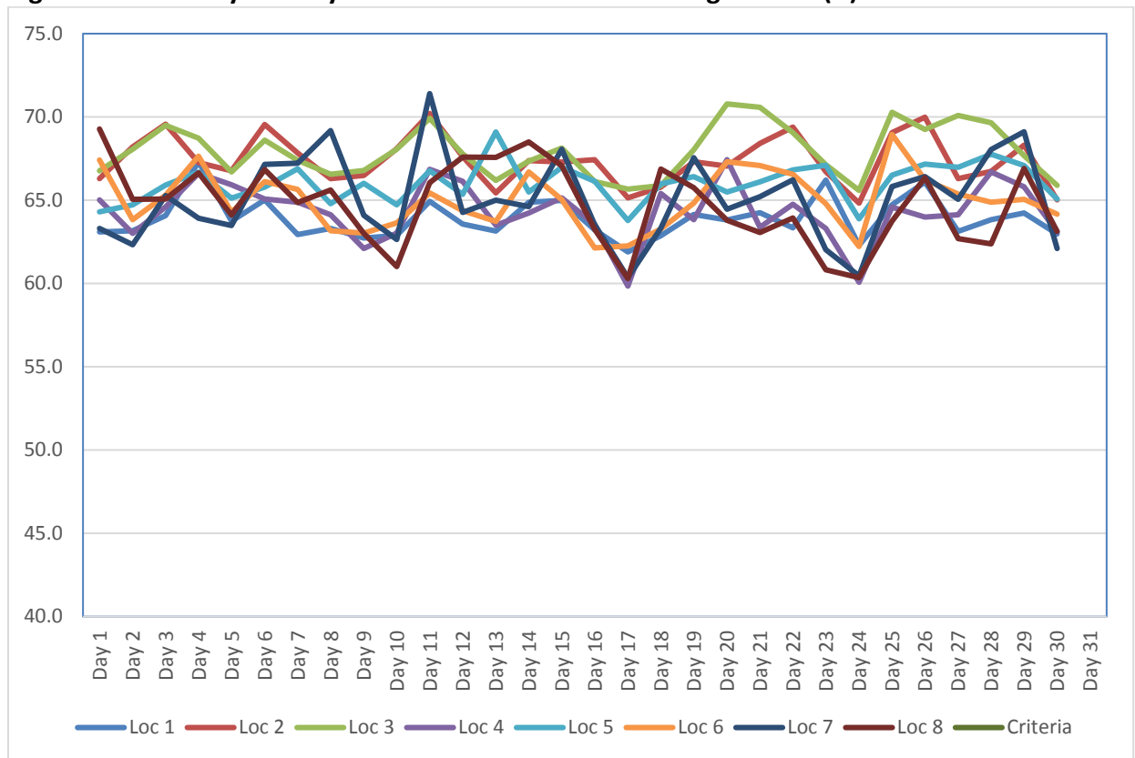
Figure 2. Summary of Daily Construction Noise Monitoring Data dB(A) – June 2018
