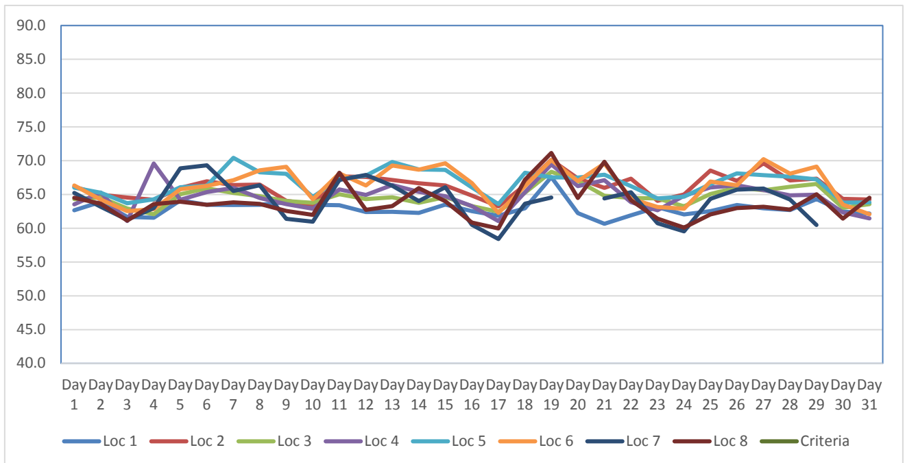
Figure 2. Summary of Daily Construction Noise Monitoring Data dB(A) – July 2016
