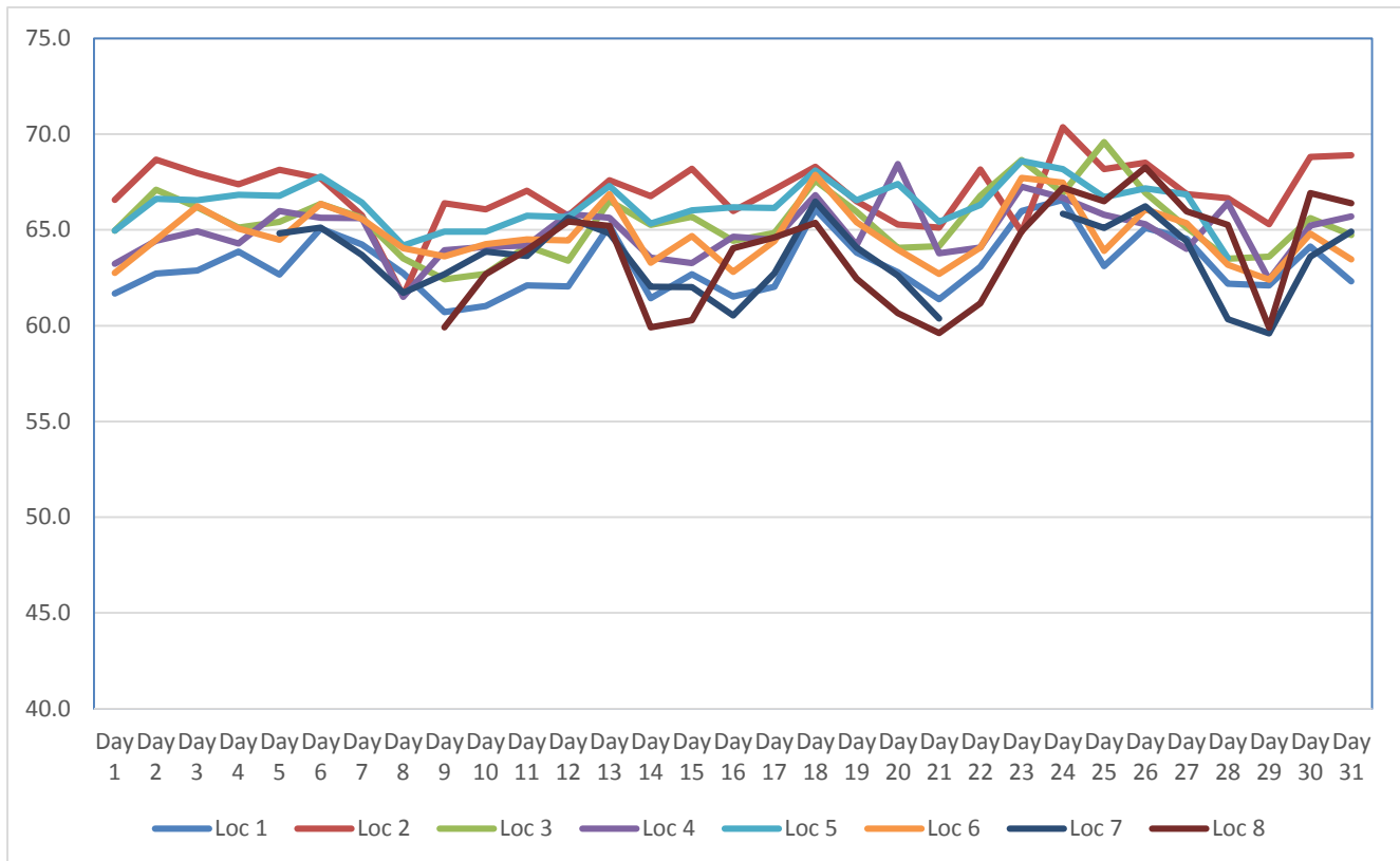
Figure 2. Summary of Daily Construction Noise Monitoring Data dB(A) – January 2017
