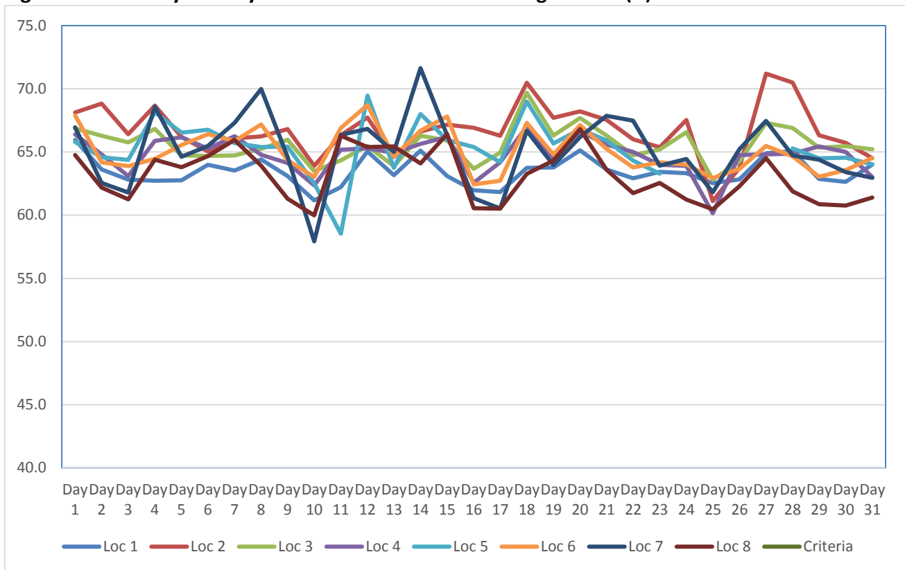
Figure 2. Summary of Daily Construction Noise Monitoring Data dB(A) – December 2017
