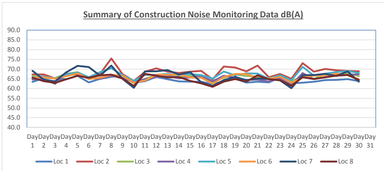
Figure 2. Summary of Daily Construction Noise Monitoring Data dB(A) – April 2016
