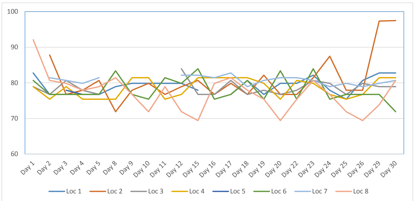
Figure 2. Summary of Construction Vibration Monitoring Data (VdB) – June 2015
