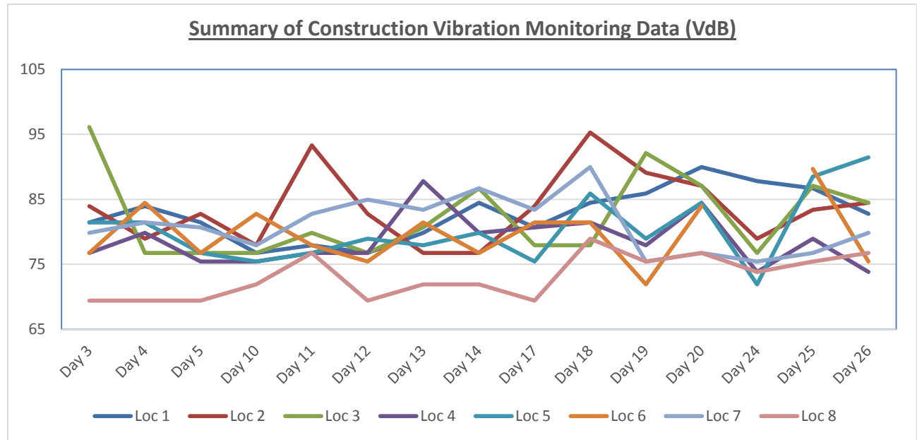
Figure 2. Summary of Construction Vibration Monitoring Data (VdB) – August 2015
