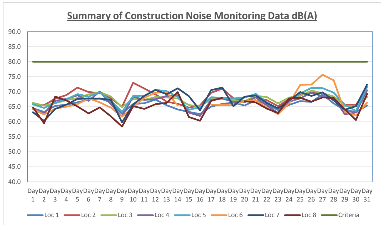
Figure 2. Summary of Daily Construction Noise Monitoring Data dB(A) – August 2015
