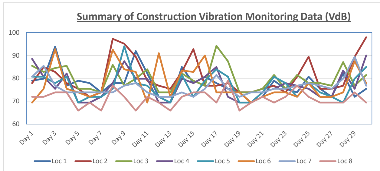
Figure 2. Summary of Construction Vibration Monitoring Data (VdB) – September 2015
