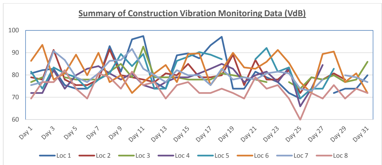
Figure 2. Summary of Construction Vibration Monitoring Data (VdB) – December 2015
