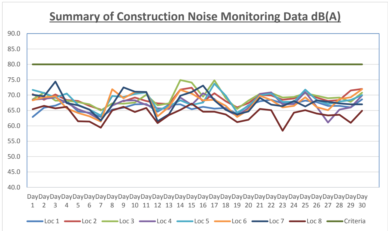
Figure 2. Summary of Daily Construction Noise Monitoring Data dB(A) – September 2015
