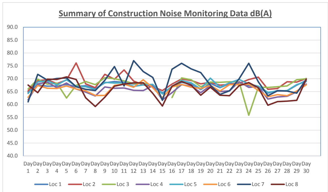
Figure 2. Summary of Daily Construction Noise Monitoring Data dB(A) – November 2015
